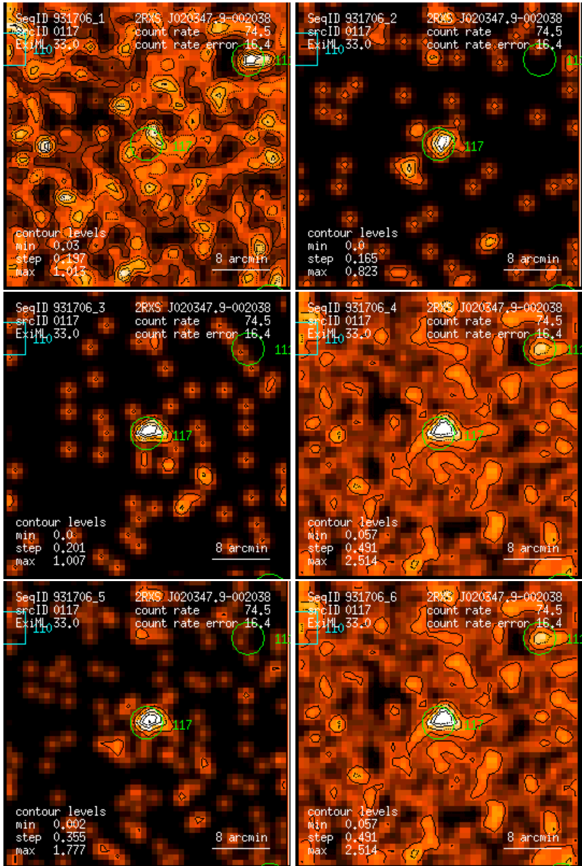
Figure 117: RASS 931706: detection 0117: band rate images, Gaussian filter: (1) PSPC channels 11 – 41, (2) 52 – 90, (3) 91 – 201, (4) 11 – 235, (5) 52 – 201, (6) 11 – 201. Broad band rates in counts/ks. Band rate contour levels in counts/ks/arcmin 2 .
