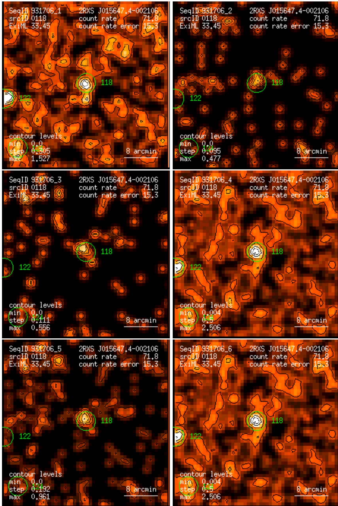
Figure 118: RASS 931706: detection 0118: band rate images, Gaussian filter: (1) PSPC channels 11 – 41, (2) 52 – 90, (3) 91 – 201, (4) 11 – 235, (5) 52 – 201, (6) 11 – 201. Broad band rates in counts/ks. Band rate contour levels in counts/ks/arcmin 2 .
