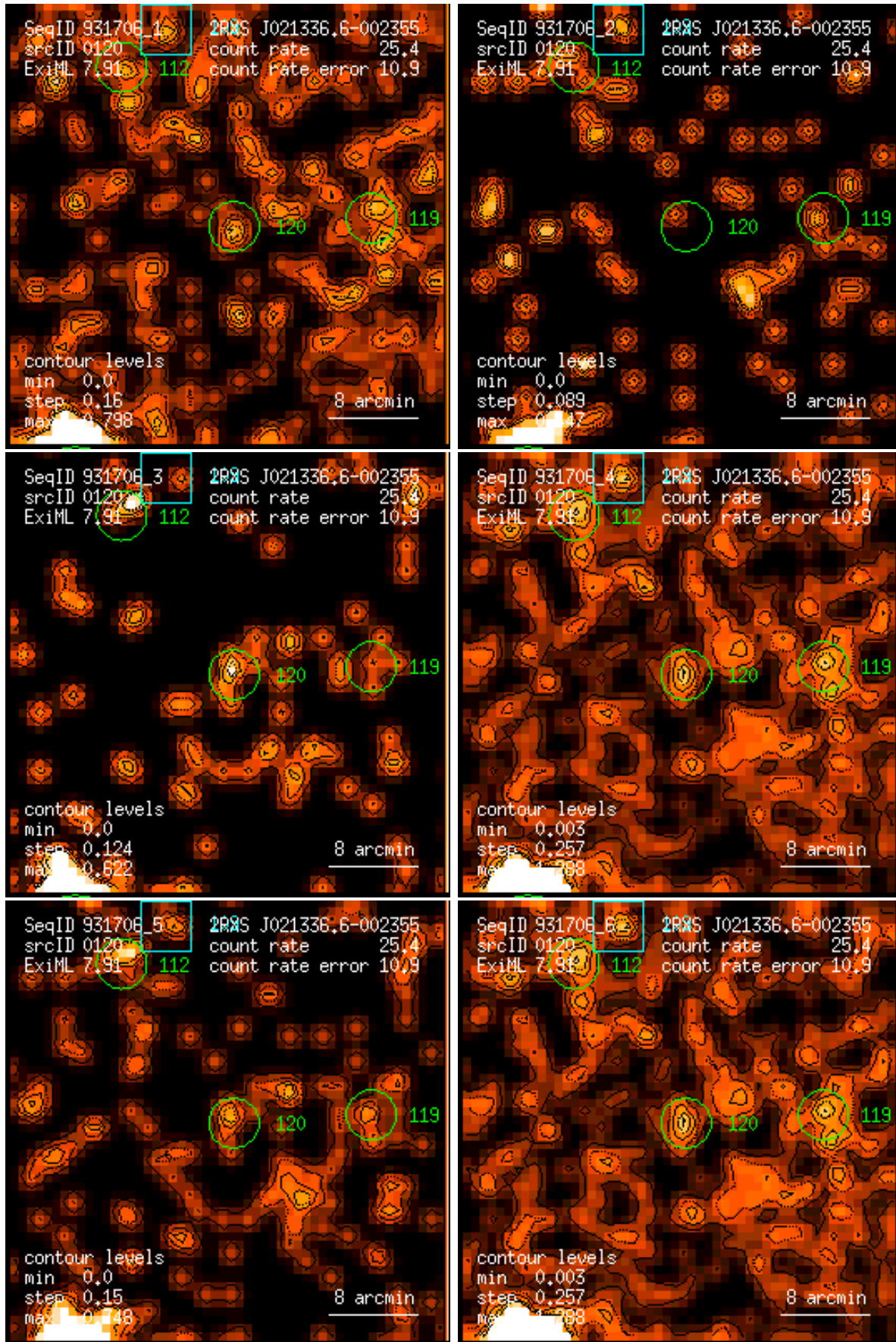
Figure 120: RASS 931706: detection 0120: band rate images, Gaussian filter: (1) PSPC channels 11 – 41, (2) 52 – 90, (3) 91 – 201, (4) 11 – 235, (5) 52 – 201, (6) 11 – 201. Broad band rates in counts/ks. Band rate contour levels in counts/ks/arcmin 2 .
