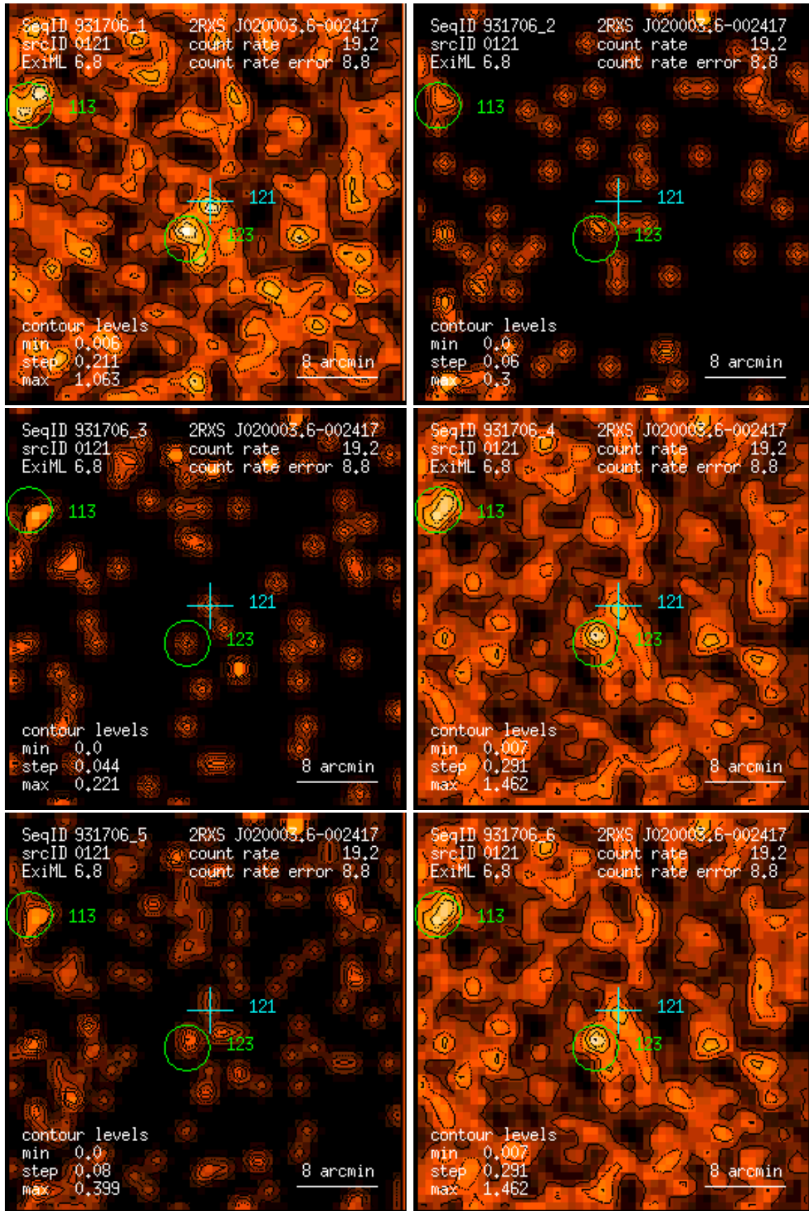
Figure 121: RASS 931706: detection 0121: band rate images, Gaussian filter: (1) PSPC channels 11 – 41, (2) 52 – 90, (3) 91 – 201, (4) 11 – 235, (5) 52 – 201, (6) 11 – 201. Broad band rates in counts/ks. Band rate contour levels in counts/ks/arcmin 2 .
