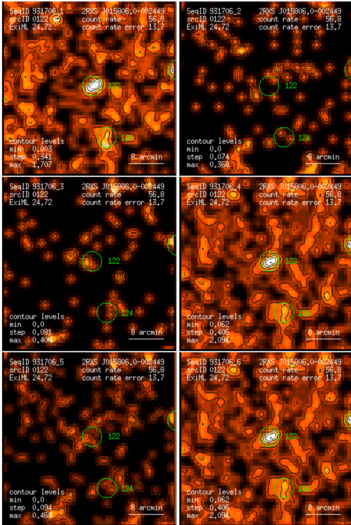
Figure 122: RASS 931706: detection 0122: band rate images, Gaussian filter: (1) PSPC channels 11 – 41, (2) 52 – 90, (3) 91 – 201, (4) 11 – 235, (5) 52 – 201, (6) 11 – 201. Broad band rates in counts/ks. Band rate contour levels in counts/ks/arcmin 2 .
