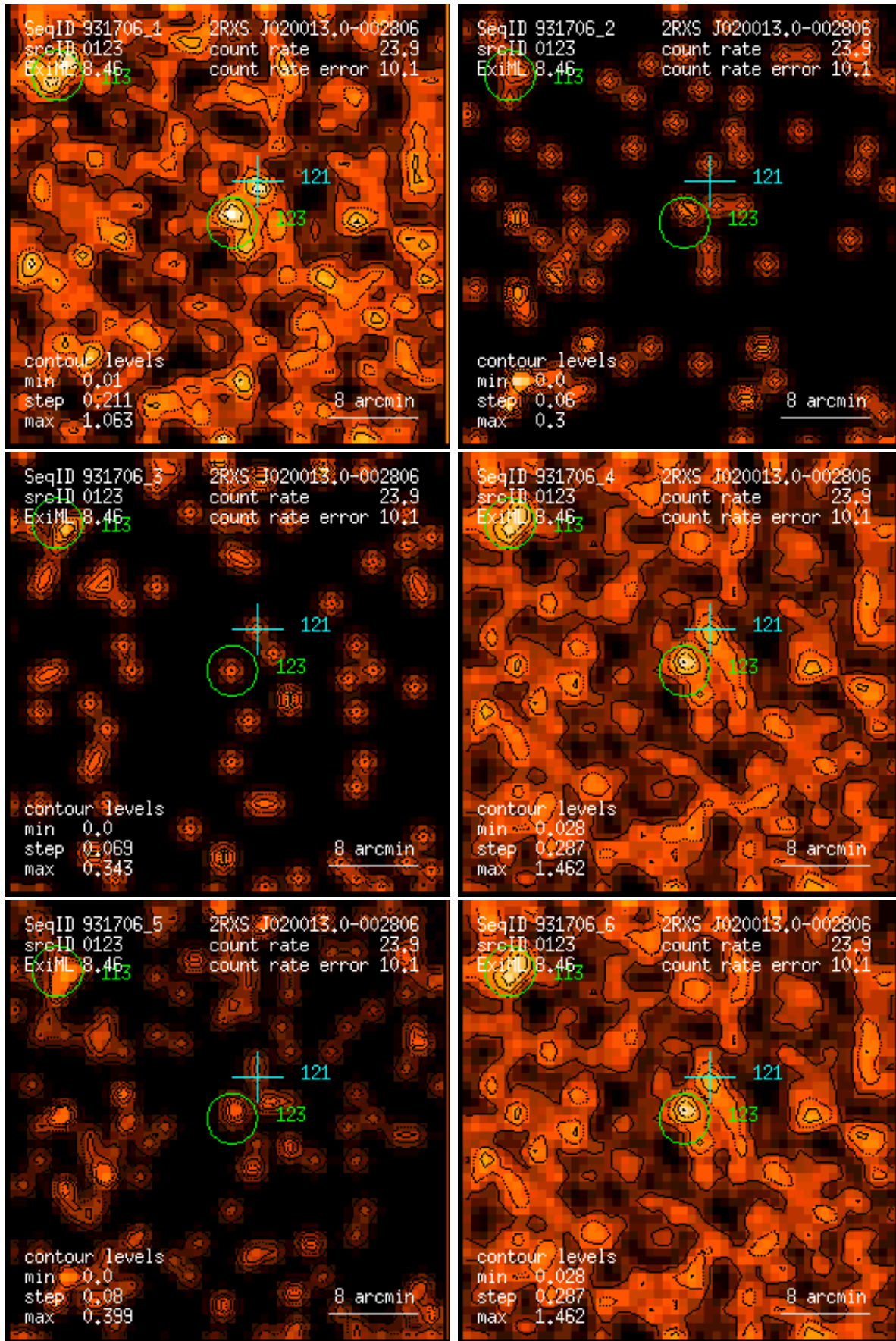
Figure 123: RASS 931706: detection 0123: band rate images, Gaussian filter: (1) PSPC channels 11 – 41, (2) 52 – 90, (3) 91 – 201, (4) 11 – 235, (5) 52 – 201, (6) 11 – 201. Broad band rates in counts/ks. Band rate contour levels in counts/ks/arcmin 2 .
