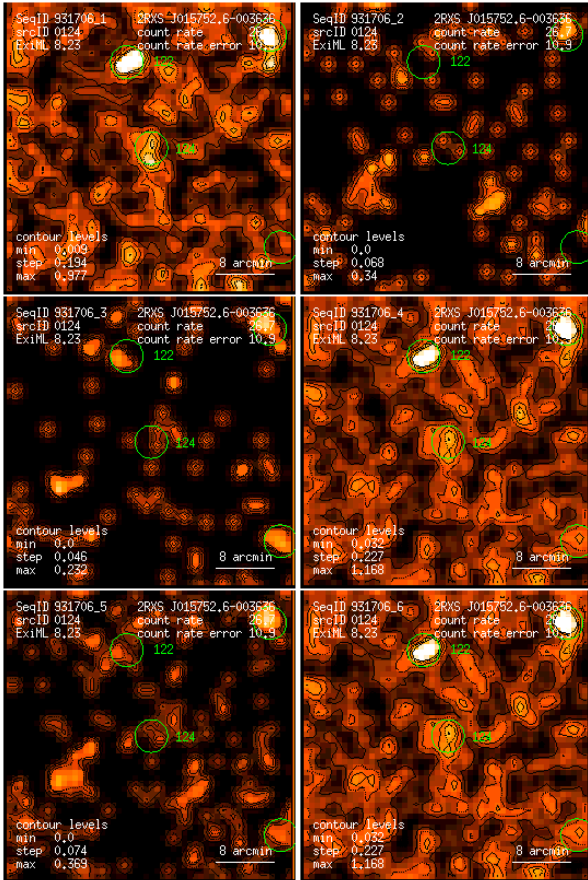
Figure 124: RASS 931706: detection 0124: band rate images, Gaussian filter: (1) PSPC channels 11 – 41, (2) 52 – 90, (3) 91 – 201, (4) 11 – 235, (5) 52 – 201, (6) 11 – 201. Broad band rates in counts/ks. Band rate contour levels in counts/ks/arcmin 2 .
