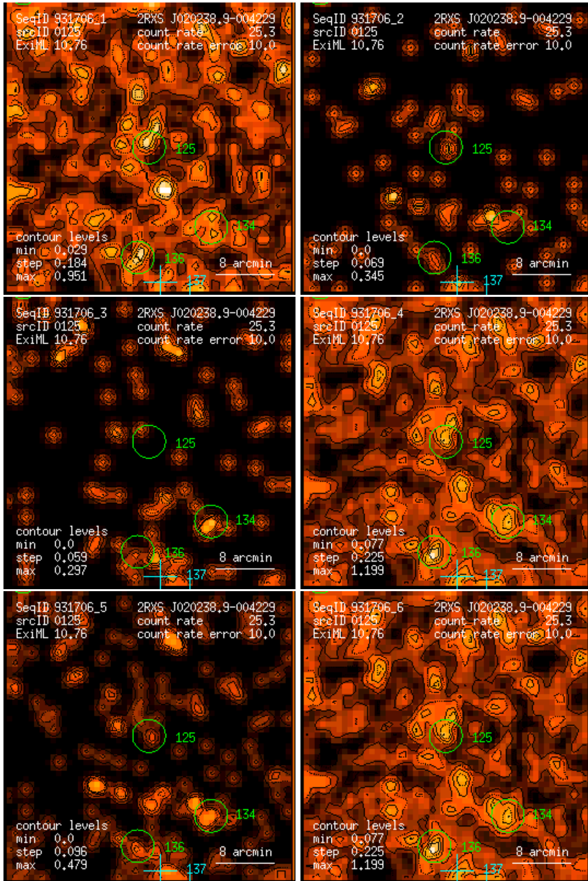
Figure 125: RASS 931706: detection 0125: band rate images, Gaussian filter: (1) PSPC channels 11 – 41, (2) 52 – 90, (3) 91 – 201, (4) 11 – 235, (5) 52 – 201, (6) 11 – 201. Broad band rates in counts/ks. Band rate contour levels in counts/ks/arcmin 2 .
