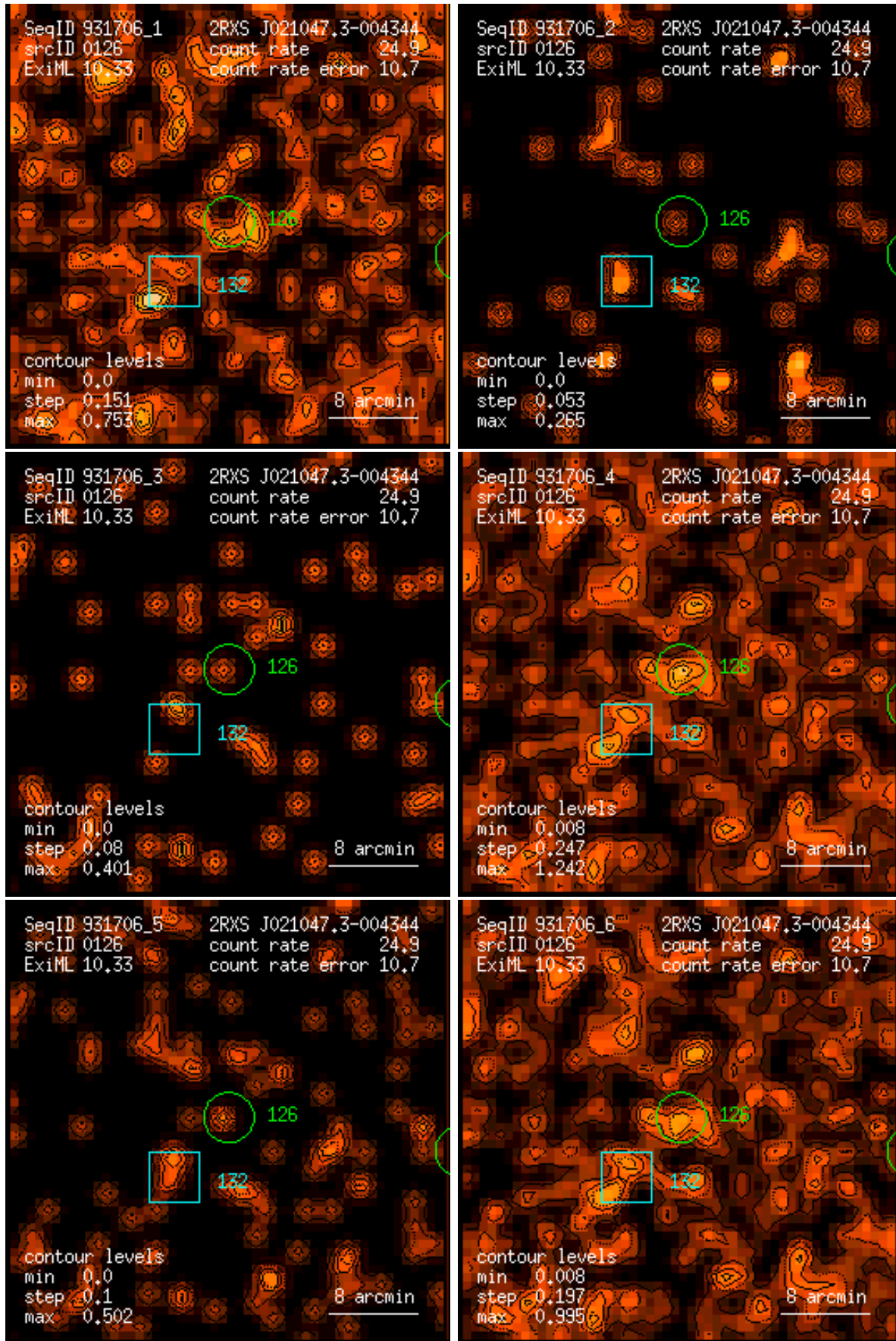
Figure 126: RASS 931706: detection 0126: band rate images, Gaussian filter: (1) PSPC channels 11 – 41, (2) 52 – 90, (3) 91 – 201, (4) 11 – 235, (5) 52 – 201, (6) 11 – 201. Broad band rates in counts/ks. Band rate contour levels in counts/ks/arcmin 2 .
