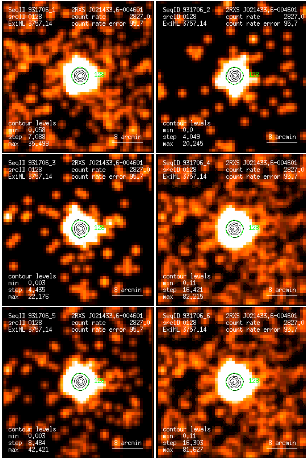
Figure 128: RASS 931706: detection 0128: band rate images, Gaussian filter: (1) PSPC channels 11 – 41, (2) 52 – 90, (3) 91 – 201, (4) 11 – 235, (5) 52 – 201, (6) 11 – 201. Broad band rates in counts/ks. Band rate contour levels in counts/ks/arcmin 2 .
