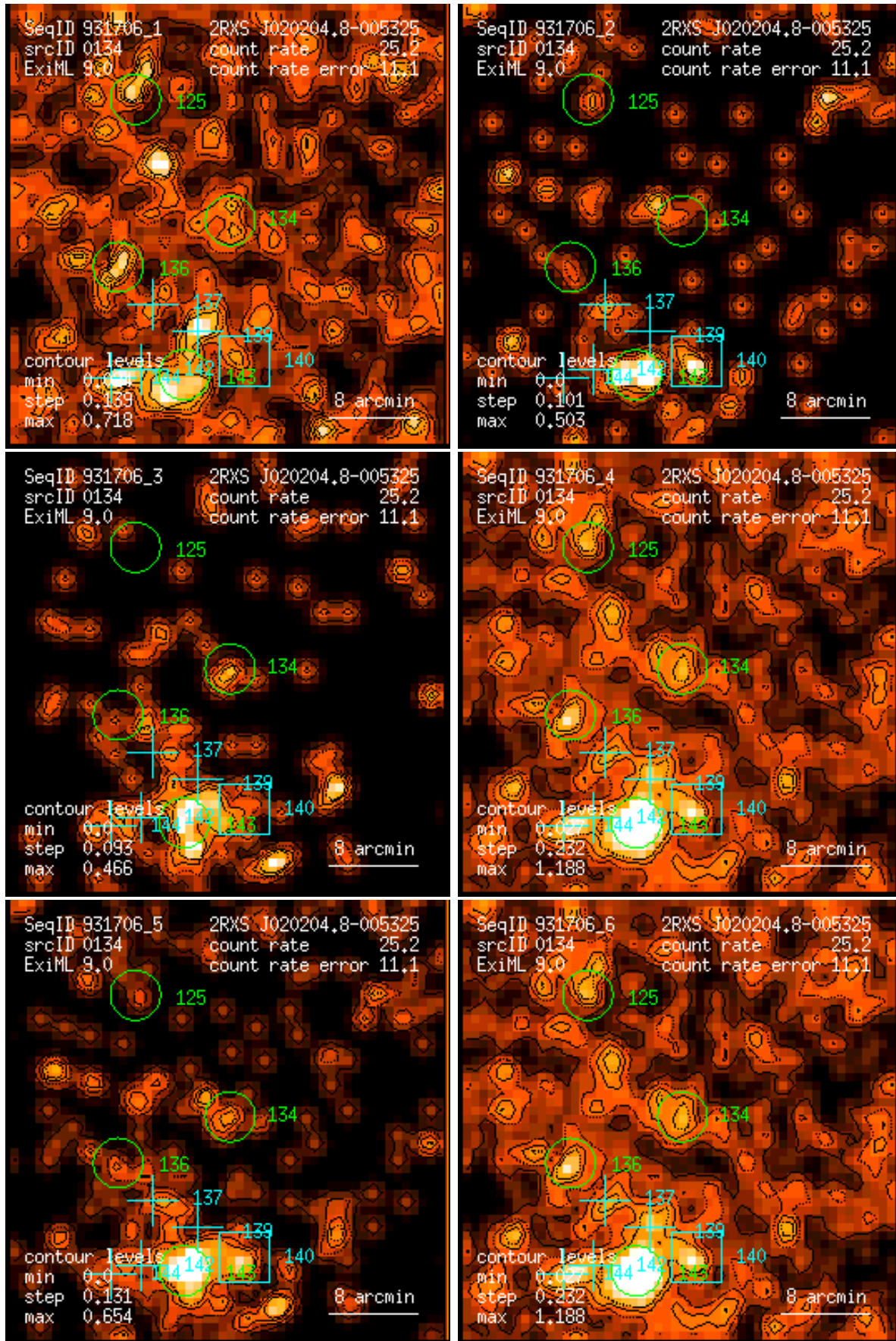
Figure 134: RASS 931706: detection 0134: band rate images, Gaussian filter: (1) PSPC channels 11 – 41, (2) 52 – 90, (3) 91 – 201, (4) 11 – 235, (5) 52 – 201, (6) 11 – 201. Broad band rates in counts/ks. Band rate contour levels in counts/ks/arcmin 2 .
