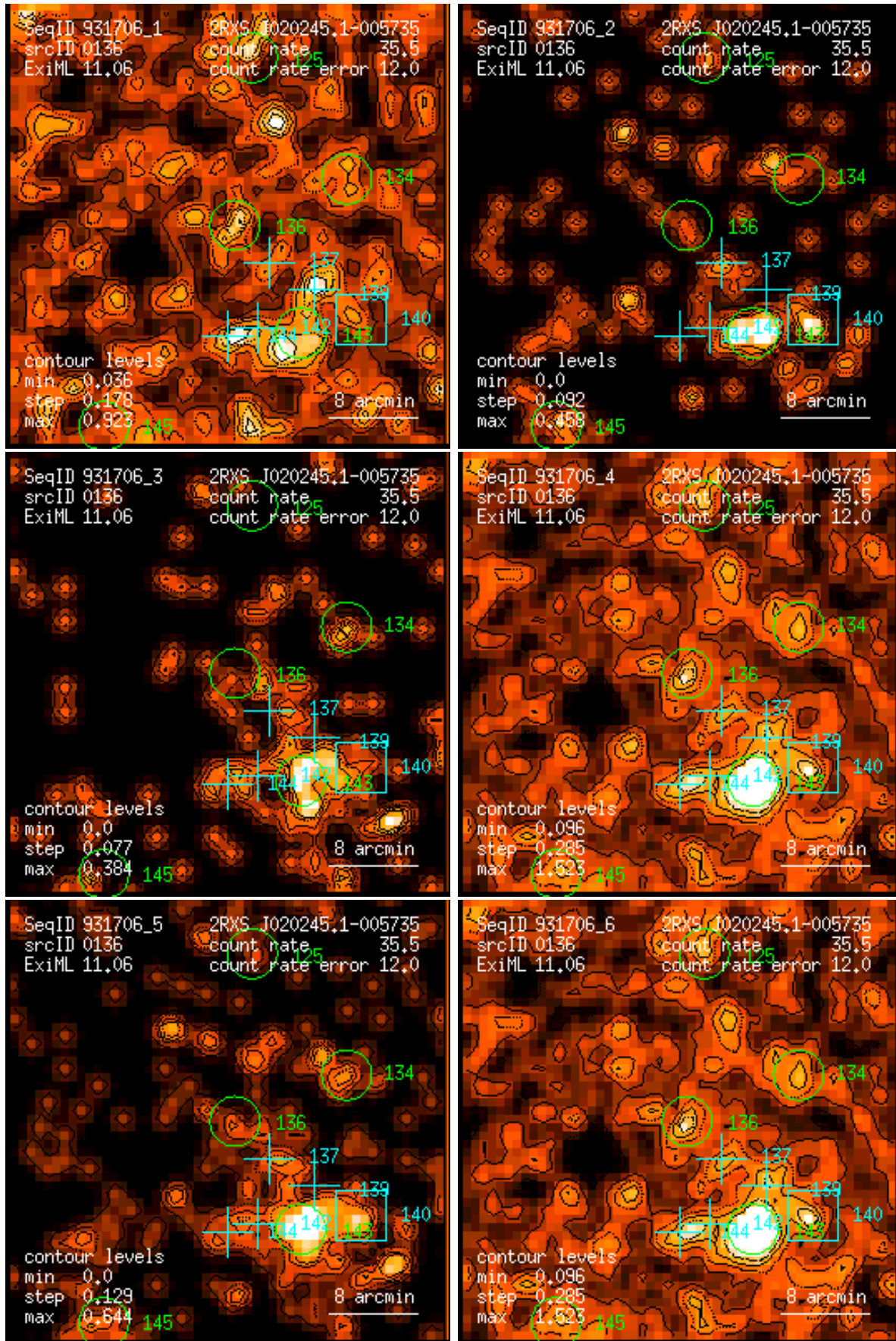
Figure 136: RASS 931706: detection 0136: band rate images, Gaussian filter: (1) PSPC channels 11 – 41, (2) 52 – 90, (3) 91 – 201, (4) 11 – 235, (5) 52 – 201, (6) 11 – 201. Broad band rates in counts/ks. Band rate contour levels in counts/ks/arcmin 2 .
