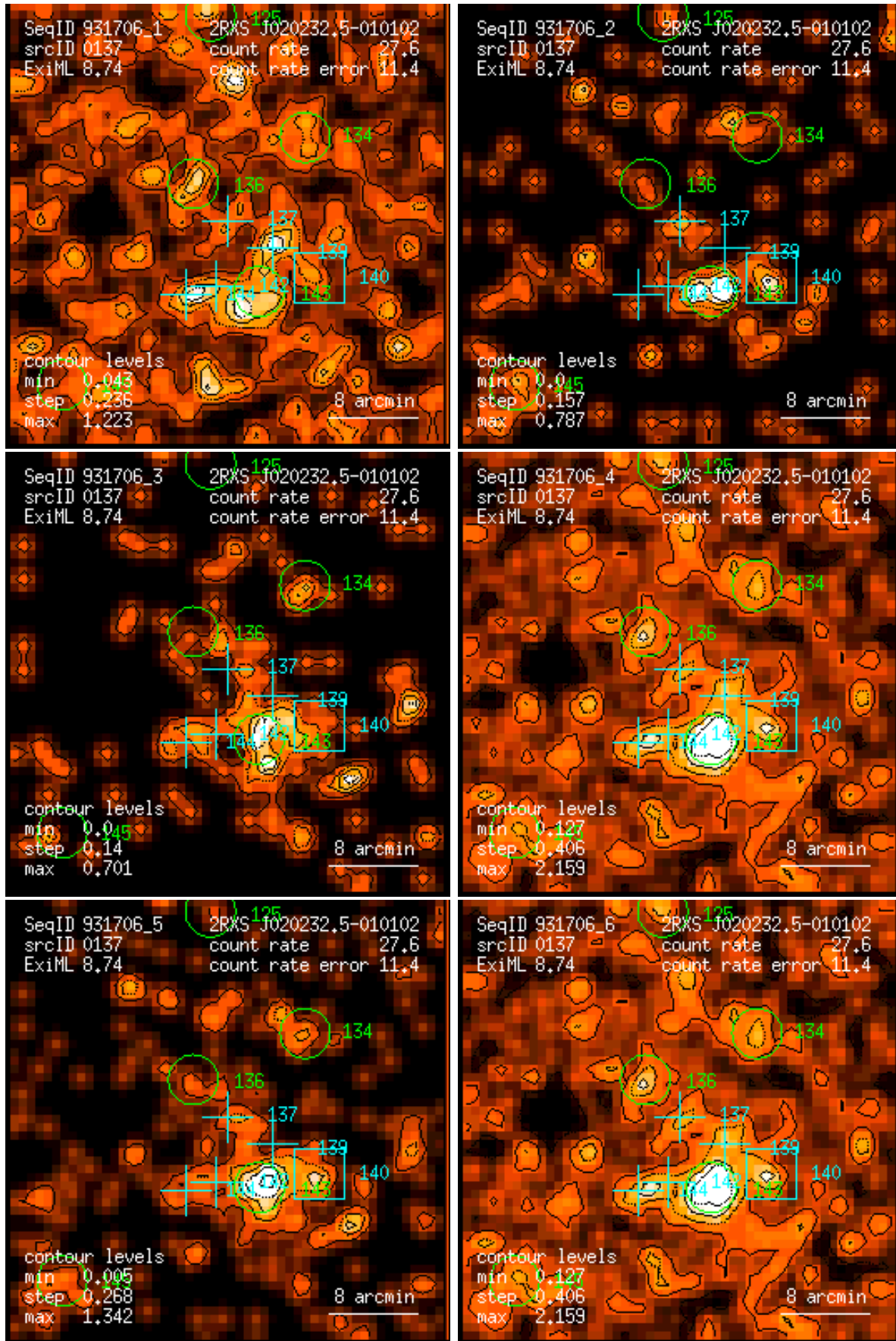
Figure 137: RASS 931706: detection 0137: band rate images, Gaussian filter: (1) PSPC channels 11 – 41, (2) 52 – 90, (3) 91 – 201, (4) 11 – 235, (5) 52 – 201, (6) 11 – 201. Broad band rates in counts/ks. Band rate contour levels in counts/ks/arcmin 2 .
