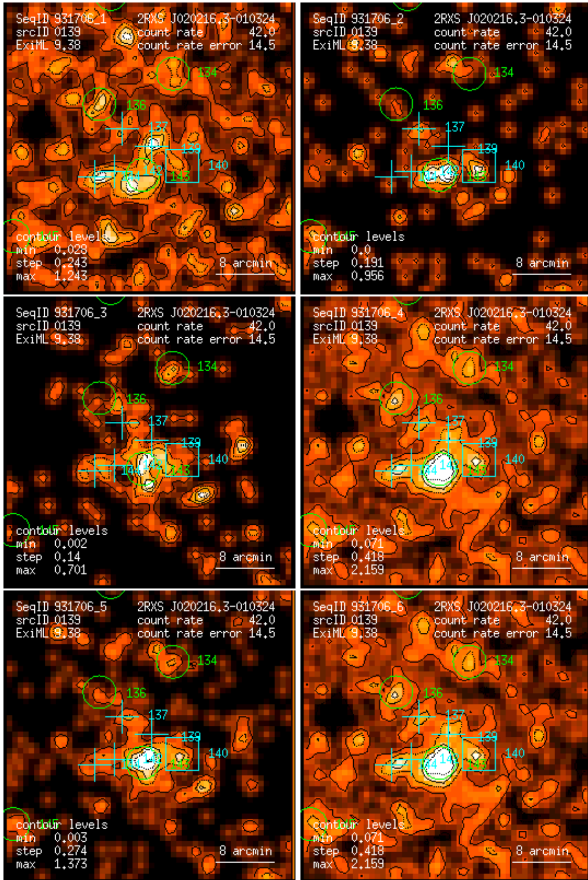
Figure 139: RASS 931706: detection 0139: band rate images, Gaussian filter: (1) PSPC channels 11 – 41, (2) 52 – 90, (3) 91 – 201, (4) 11 – 235, (5) 52 – 201, (6) 11 – 201. Broad band rates in counts/ks. Band rate contour levels in counts/ks/arcmin 2 .
