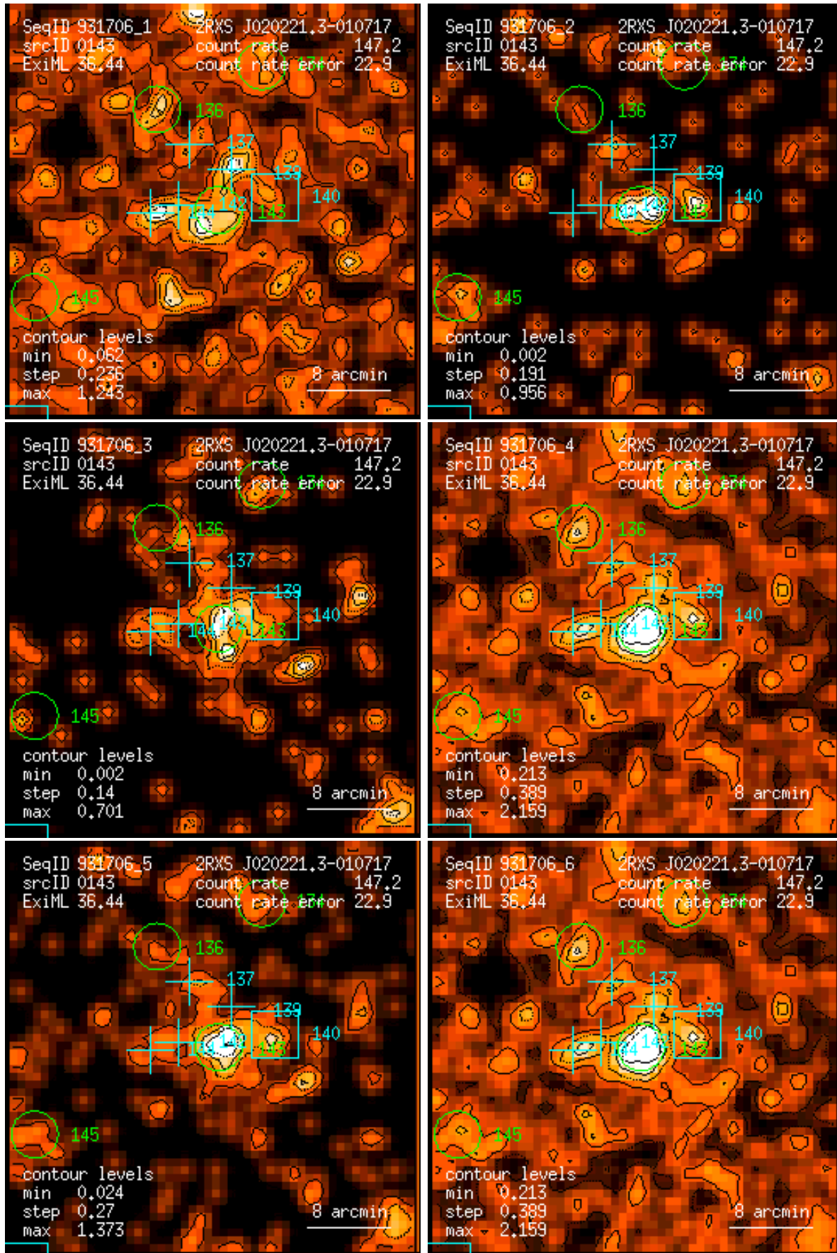
Figure 143: RASS 931706: detection 0143: band rate images, Gaussian filter: (1) PSPC channels 11 – 41, (2) 52 – 90, (3) 91 – 201, (4) 11 – 235, (5) 52 – 201, (6) 11 – 201. Broad band rates in counts/ks. Band rate contour levels in counts/ks/arcmin 2 .
