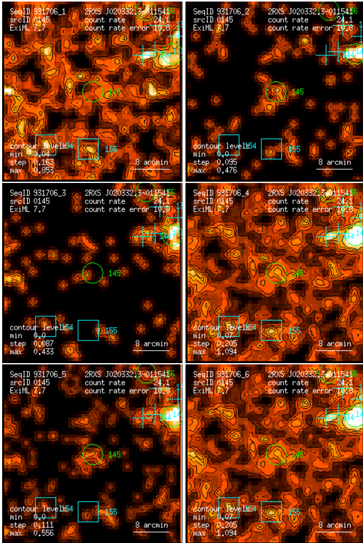
Figure 145: RASS 931706: detection 0145: band rate images, Gaussian filter: (1) PSPC channels 11 – 41, (2) 52 – 90, (3) 91 – 201, (4) 11 – 235, (5) 52 – 201, (6) 11 – 201. Broad band rates in counts/ks. Band rate contour levels in counts/ks/arcmin 2 .
