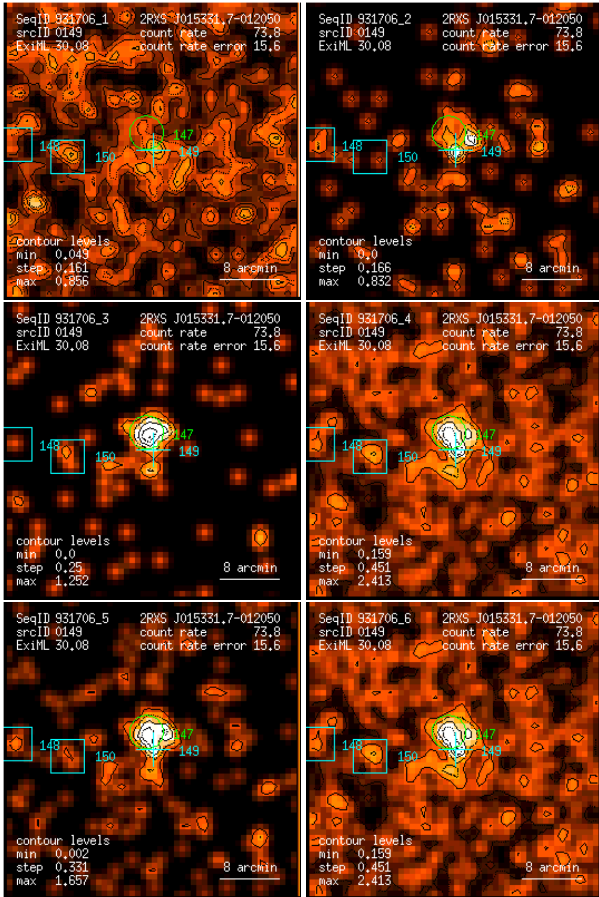
Figure 149: RASS 931706: detection 0149: band rate images, Gaussian filter: (1) PSPC channels 11 – 41, (2) 52 – 90, (3) 91 – 201, (4) 11 – 235, (5) 52 – 201, (6) 11 – 201. Broad band rates in counts/ks. Band rate contour levels in counts/ks/arcmin 2 .
