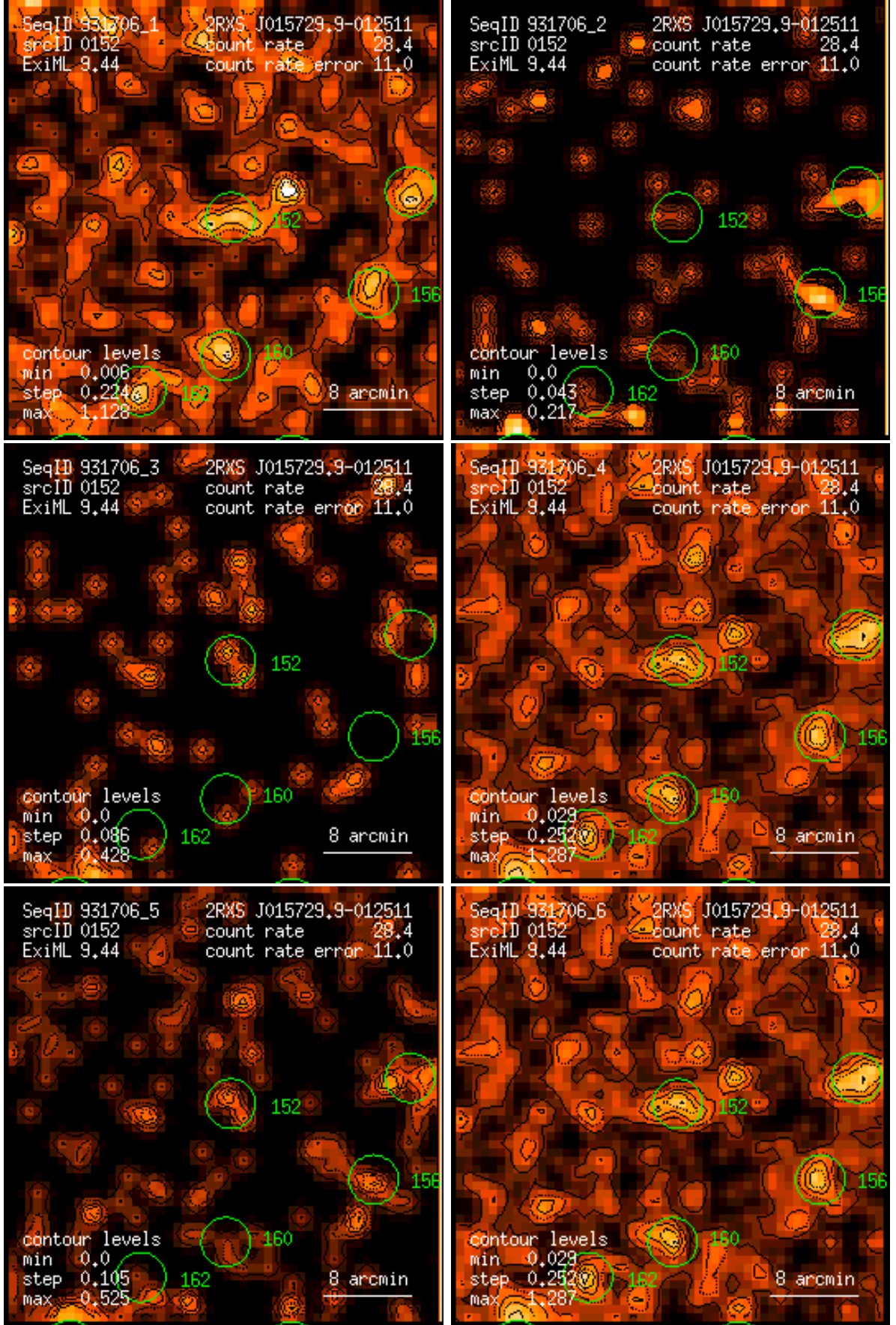
Figure 152: RASS 931706: detection 0152: band rate images, Gaussian filter: (1) PSPC channels 11 – 41, (2) 52 – 90, (3) 91 – 201, (4) 11 – 235, (5) 52 – 201, (6) 11 – 201. Broad band rates in counts/ks. Band rate contour levels in counts/ks/arcmin 2 .
