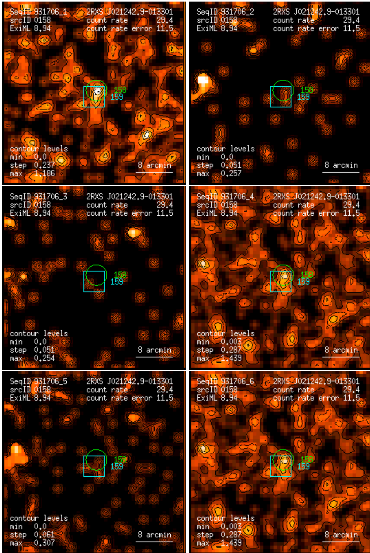
Figure 158: RASS 931706: detection 0158: band rate images, Gaussian filter: (1) PSPC channels 11 – 41, (2) 52 – 90, (3) 91 – 201, (4) 11 – 235, (5) 52 – 201, (6) 11 – 201. Broad band rates in counts/ks. Band rate contour levels in counts/ks/arcmin 2 .
