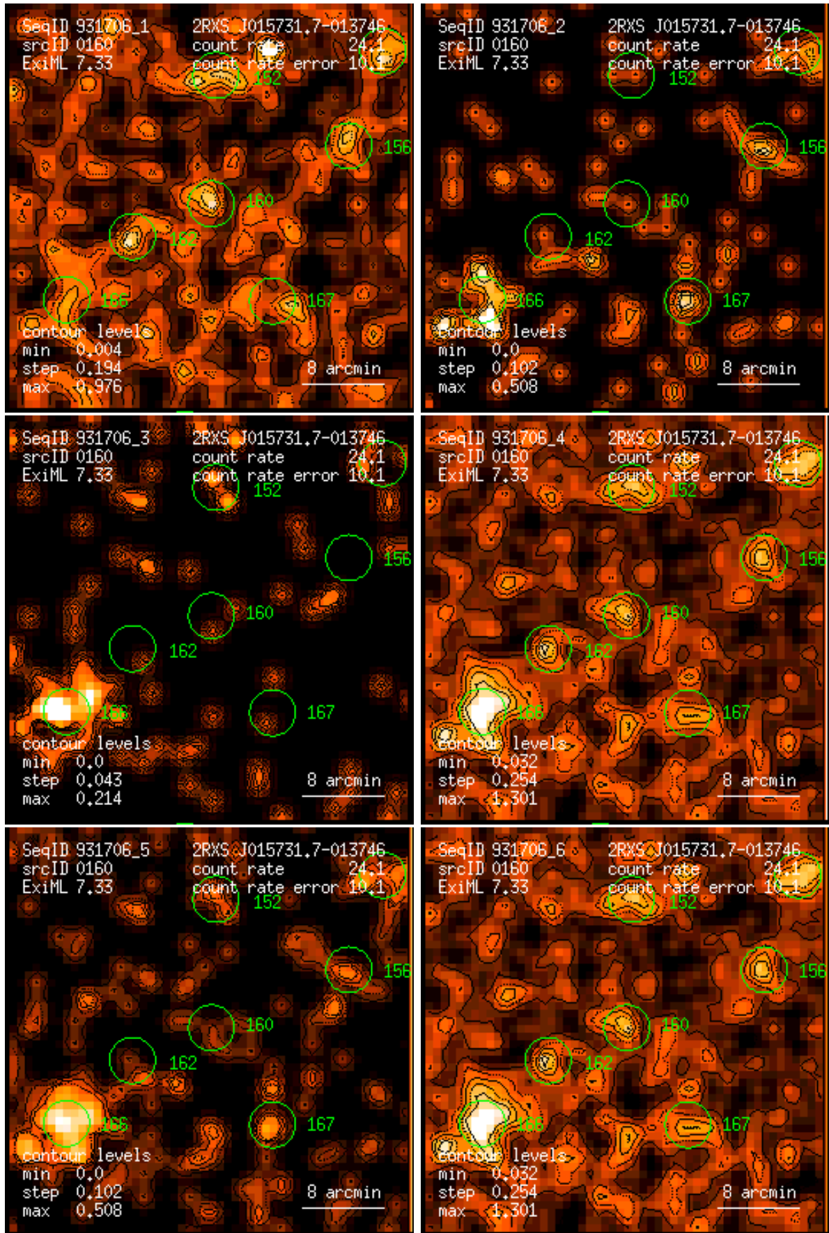
Figure 160: RASS 931706: detection 0160: band rate images, Gaussian filter: (1) PSPC channels 11 – 41, (2) 52 – 90, (3) 91 – 201, (4) 11 – 235, (5) 52 – 201, (6) 11 – 201. Broad band rates in counts/ks. Band rate contour levels in counts/ks/arcmin 2 .
