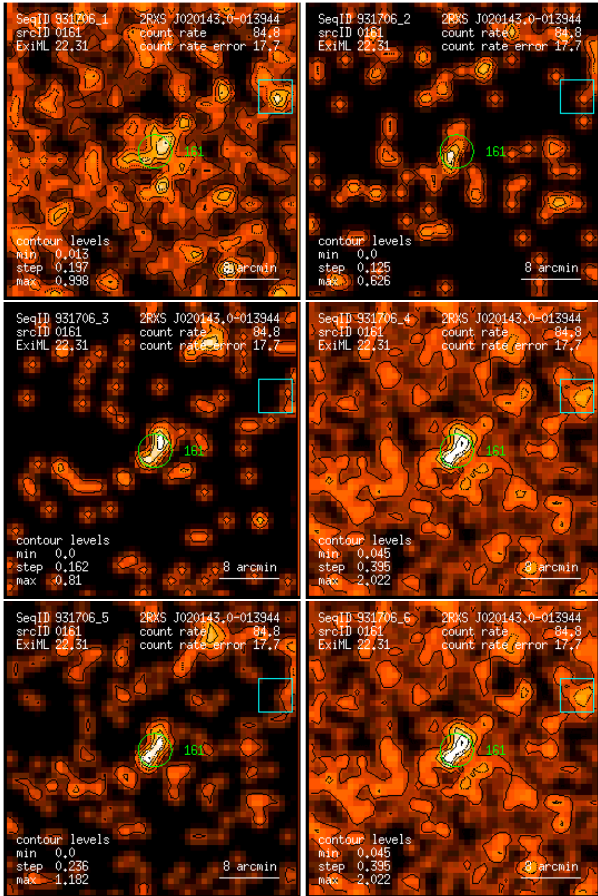
Figure 161: RASS 931706: detection 0161: band rate images, Gaussian filter: (1) PSPC channels 11 – 41, (2) 52 – 90, (3) 91 – 201, (4) 11 – 235, (5) 52 – 201, (6) 11 – 201. Broad band rates in counts/ks. Band rate contour levels in counts/ks/arcmin 2 .
