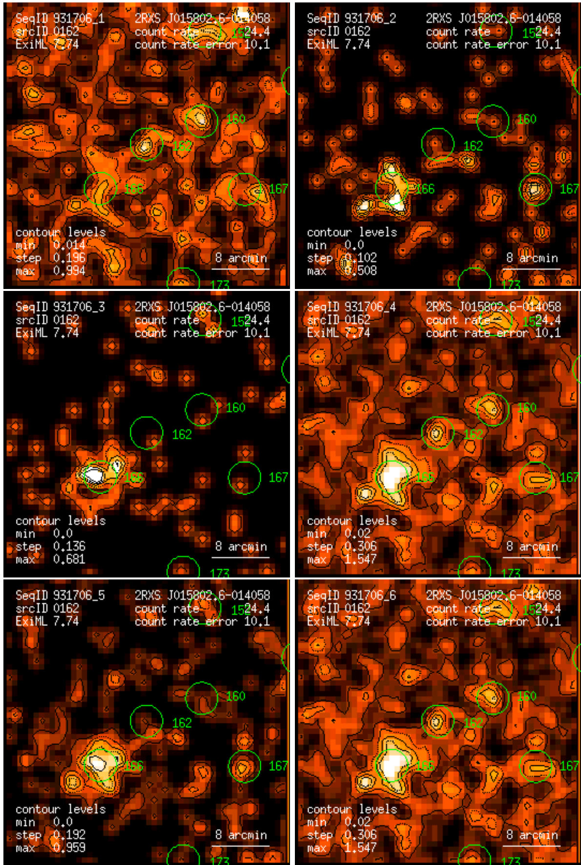
Figure 162: RASS 931706: detection 0162: band rate images, Gaussian filter: (1) PSPC channels 11 – 41, (2) 52 – 90, (3) 91 – 201, (4) 11 – 235, (5) 52 – 201, (6) 11 – 201. Broad band rates in counts/ks. Band rate contour levels in counts/ks/arcmin 2 .
