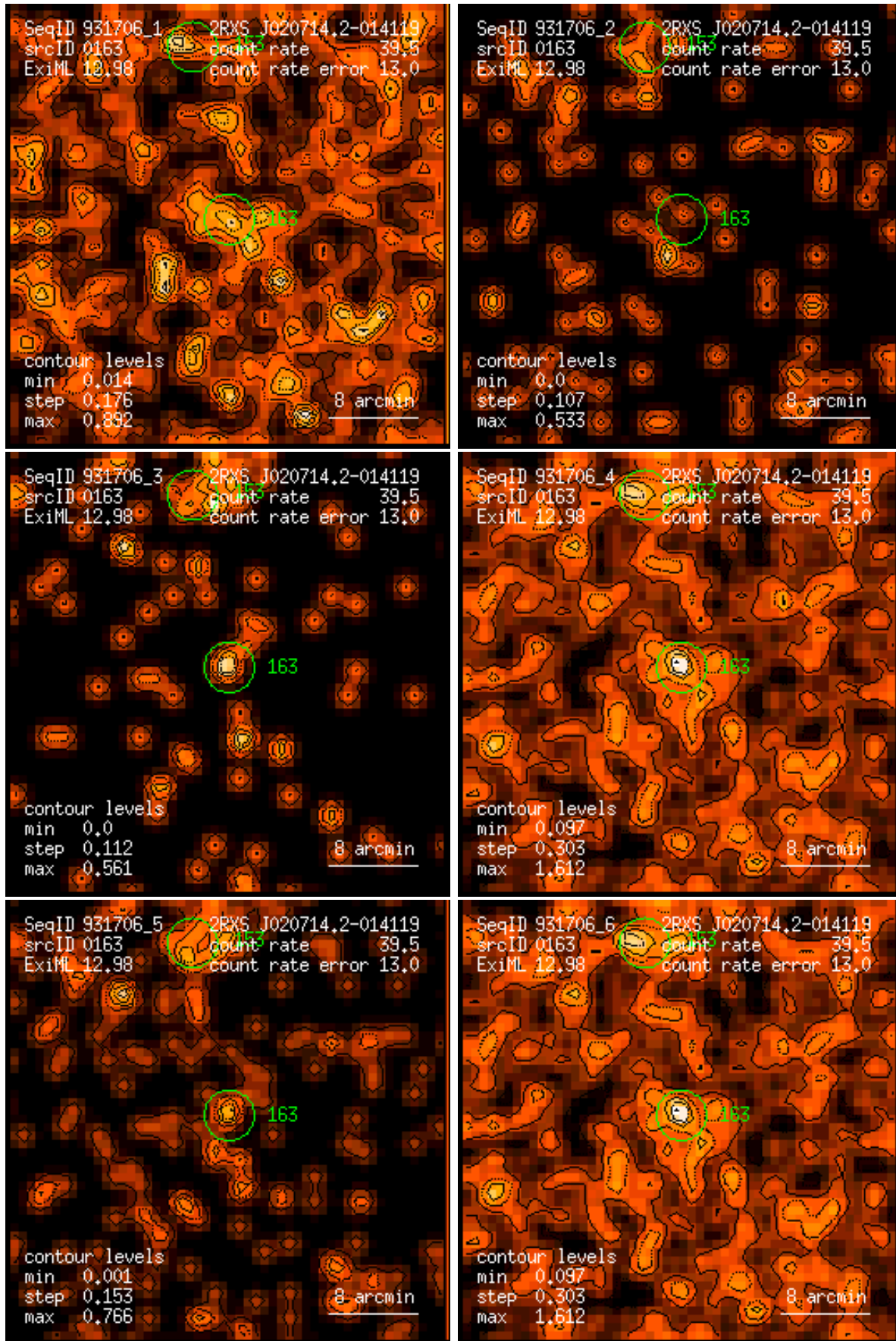
Figure 163: RASS 931706: detection 0163: band rate images, Gaussian filter: (1) PSPC channels 11 – 41, (2) 52 – 90, (3) 91 – 201, (4) 11 – 235, (5) 52 – 201, (6) 11 – 201. Broad band rates in counts/ks. Band rate contour levels in counts/ks/arcmin 2 .
