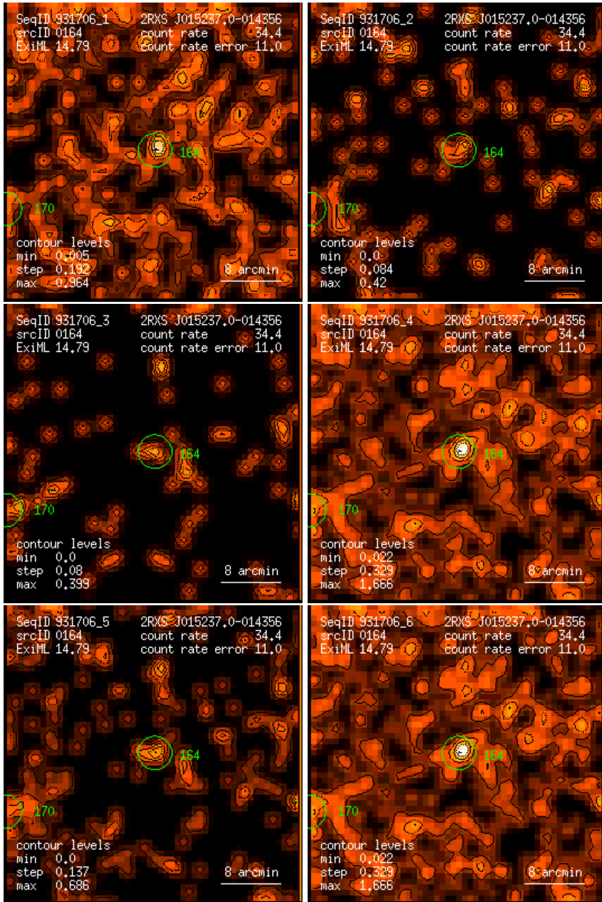
Figure 164: RASS 931706: detection 0164: band rate images, Gaussian filter: (1) PSPC channels 11 – 41, (2) 52 – 90, (3) 91 – 201, (4) 11 – 235, (5) 52 – 201, (6) 11 – 201. Broad band rates in counts/ks. Band rate contour levels in counts/ks/arcmin 2 .
