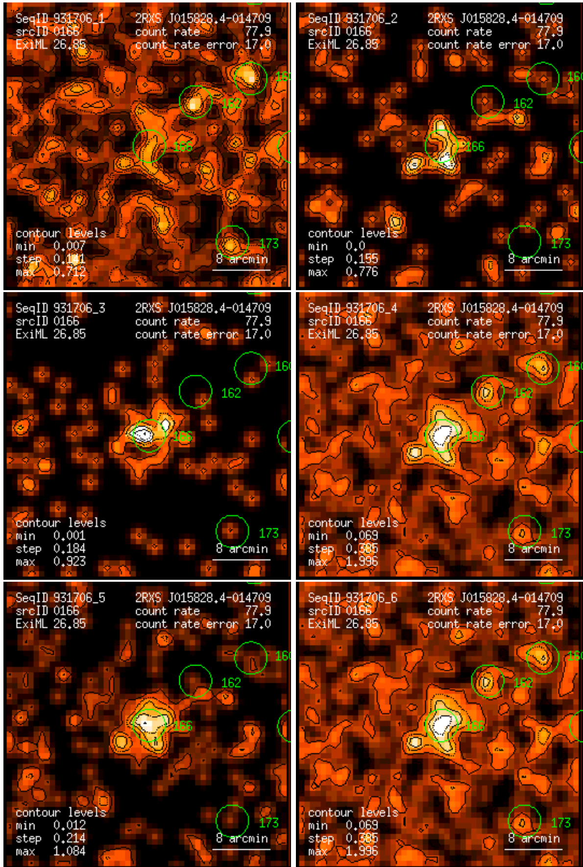
Figure 166: RASS 931706: detection 0166: band rate images, Gaussian filter: (1) PSPC channels 11 – 41, (2) 52 – 90, (3) 91 – 201, (4) 11 – 235, (5) 52 – 201, (6) 11 – 201. Broad band rates in counts/ks. Band rate contour levels in counts/ks/arcmin 2 .
