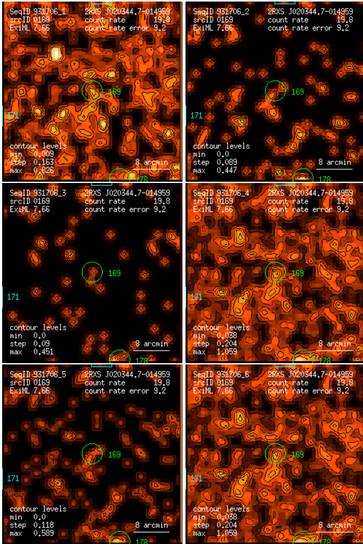
Figure 169: RASS 931706: detection 0169: band rate images, Gaussian filter: (1) PSPC channels 11 – 41, (2) 52 – 90, (3) 91 – 201, (4) 11 – 235, (5) 52 – 201, (6) 11 – 201. Broad band rates in counts/ks. Band rate contour levels in counts/ks/arcmin 2 .
