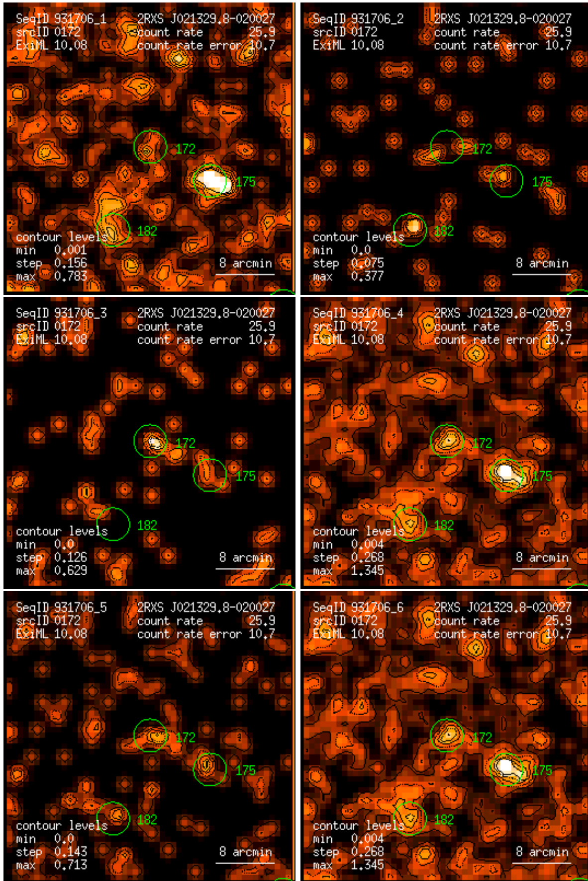
Figure 172: RASS 931706: detection 0172: band rate images, Gaussian filter: (1) PSPC channels 11 – 41, (2) 52 – 90, (3) 91 – 201, (4) 11 – 235, (5) 52 – 201, (6) 11 – 201. Broad band rates in counts/ks. Band rate contour levels in counts/ks/arcmin 2 .
