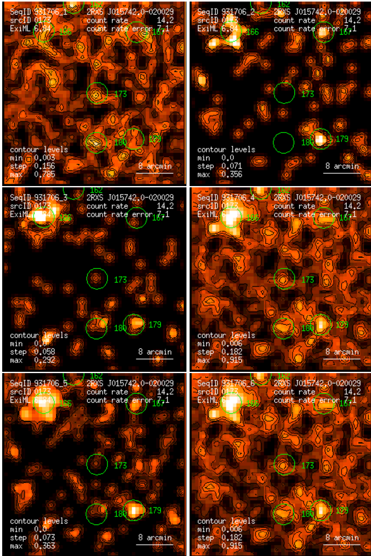
Figure 173: RASS 931706: detection 0173: band rate images, Gaussian filter: (1) PSPC channels 11 – 41, (2) 52 – 90, (3) 91 – 201, (4) 11 – 235, (5) 52 – 201, (6) 11 – 201. Broad band rates in counts/ks. Band rate contour levels in counts/ks/arcmin 2 .
