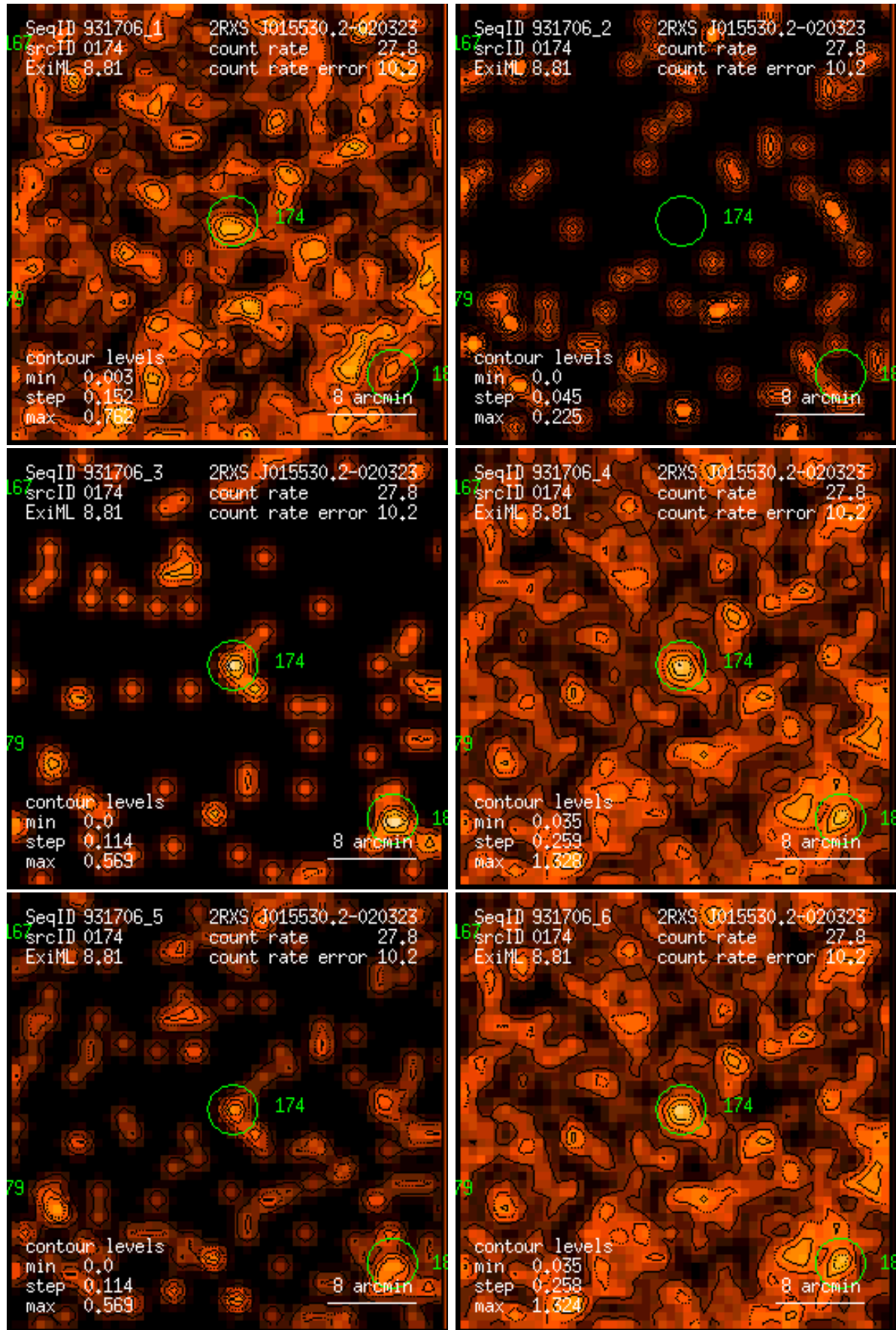
Figure 174: RASS 931706: detection 0174: band rate images, Gaussian filter: (1) PSPC channels 11 – 41, (2) 52 – 90, (3) 91 – 201, (4) 11 – 235, (5) 52 – 201, (6) 11 – 201. Broad band rates in counts/ks. Band rate contour levels in counts/ks/arcmin 2 .
