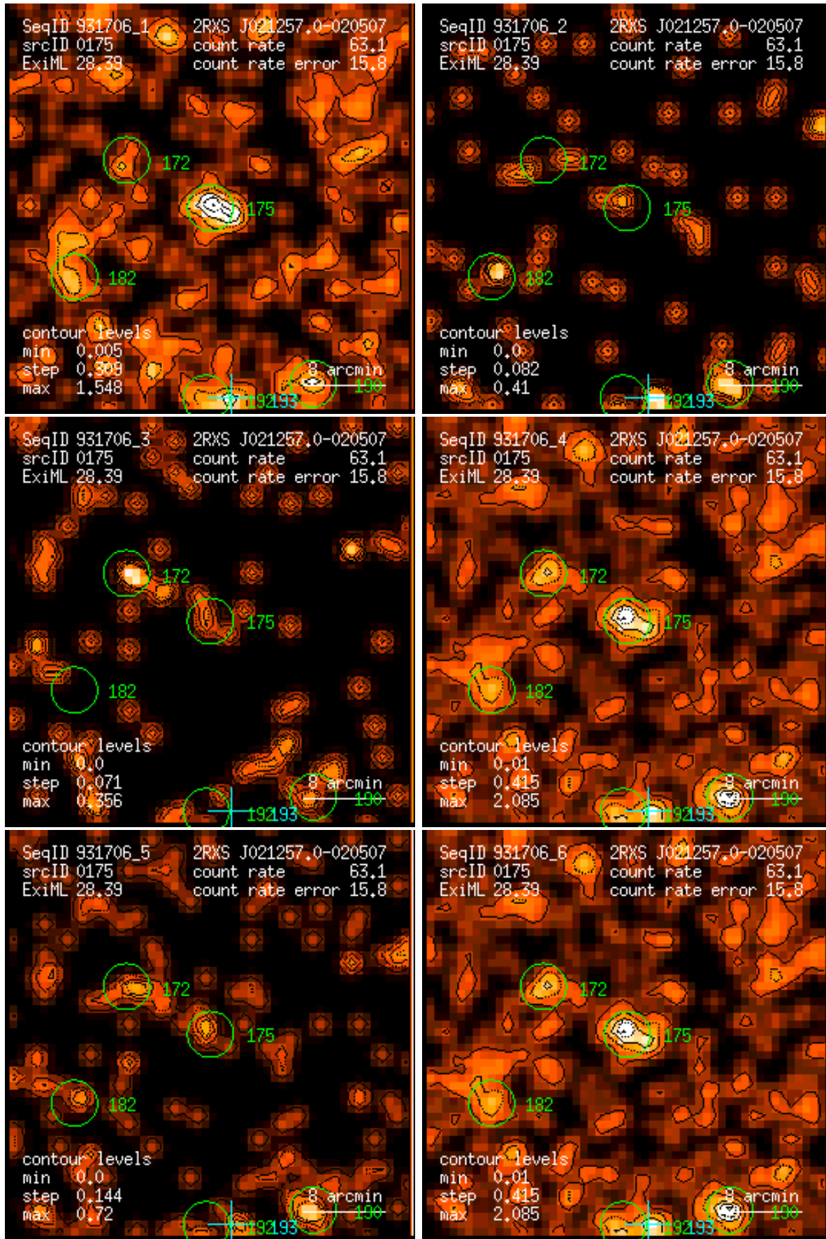
Figure 175: RASS 931706: detection 0175: band rate images, Gaussian filter: (1) PSPC channels 11 – 41, (2) 52 – 90, (3) 91 – 201, (4) 11 – 235, (5) 52 – 201, (6) 11 – 201. Broad band rates in counts/ks. Band rate contour levels in counts/ks/arcmin 2 .
