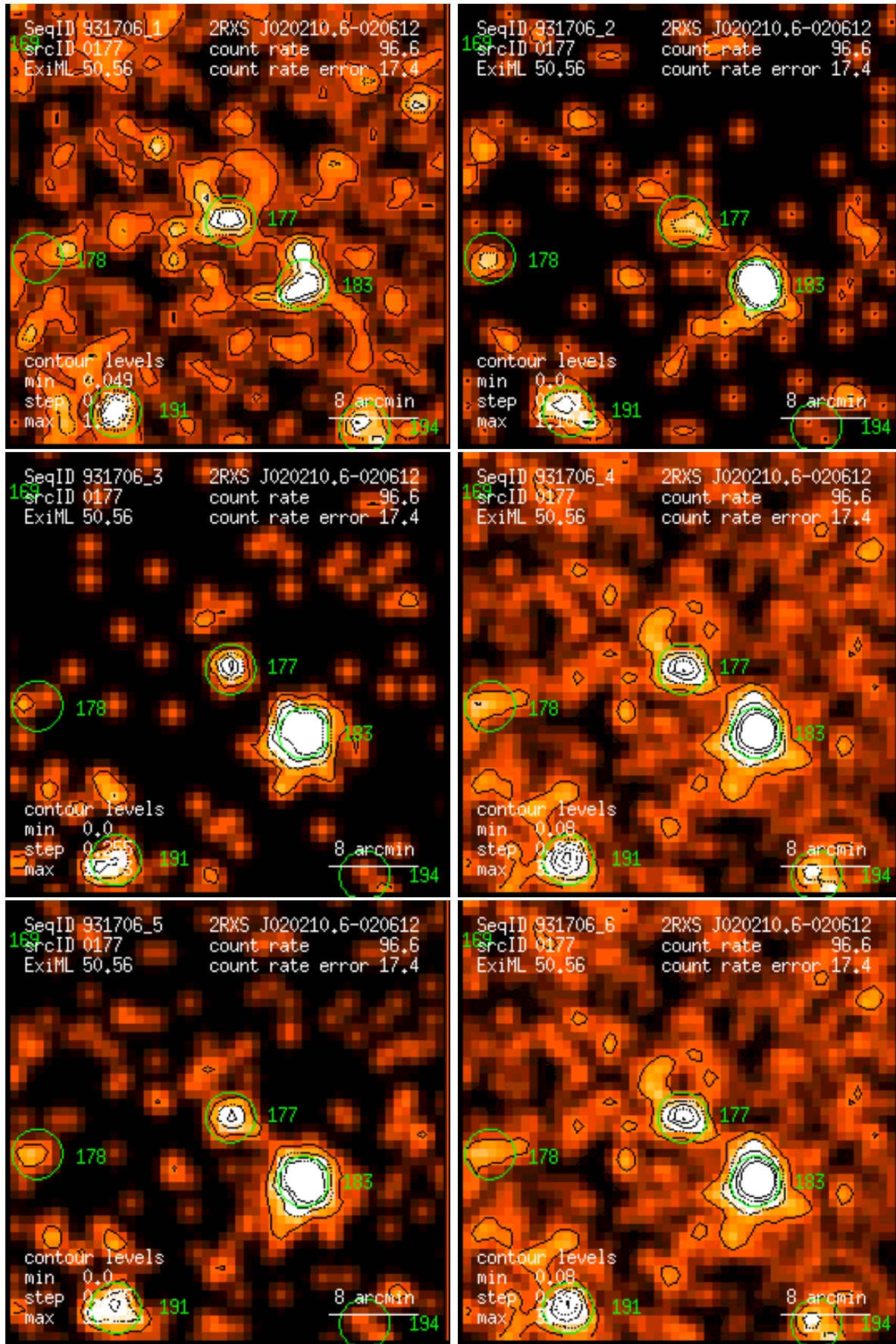
Figure 177: RASS 931706: detection 0177: band rate images, Gaussian filter: (1) PSPC channels 11 – 41, (2) 52 – 90, (3) 91 – 201, (4) 11 – 235, (5) 52 – 201, (6) 11 – 201. Broad band rates in counts/ks. Band rate contour levels in counts/ks/arcmin 2 .
