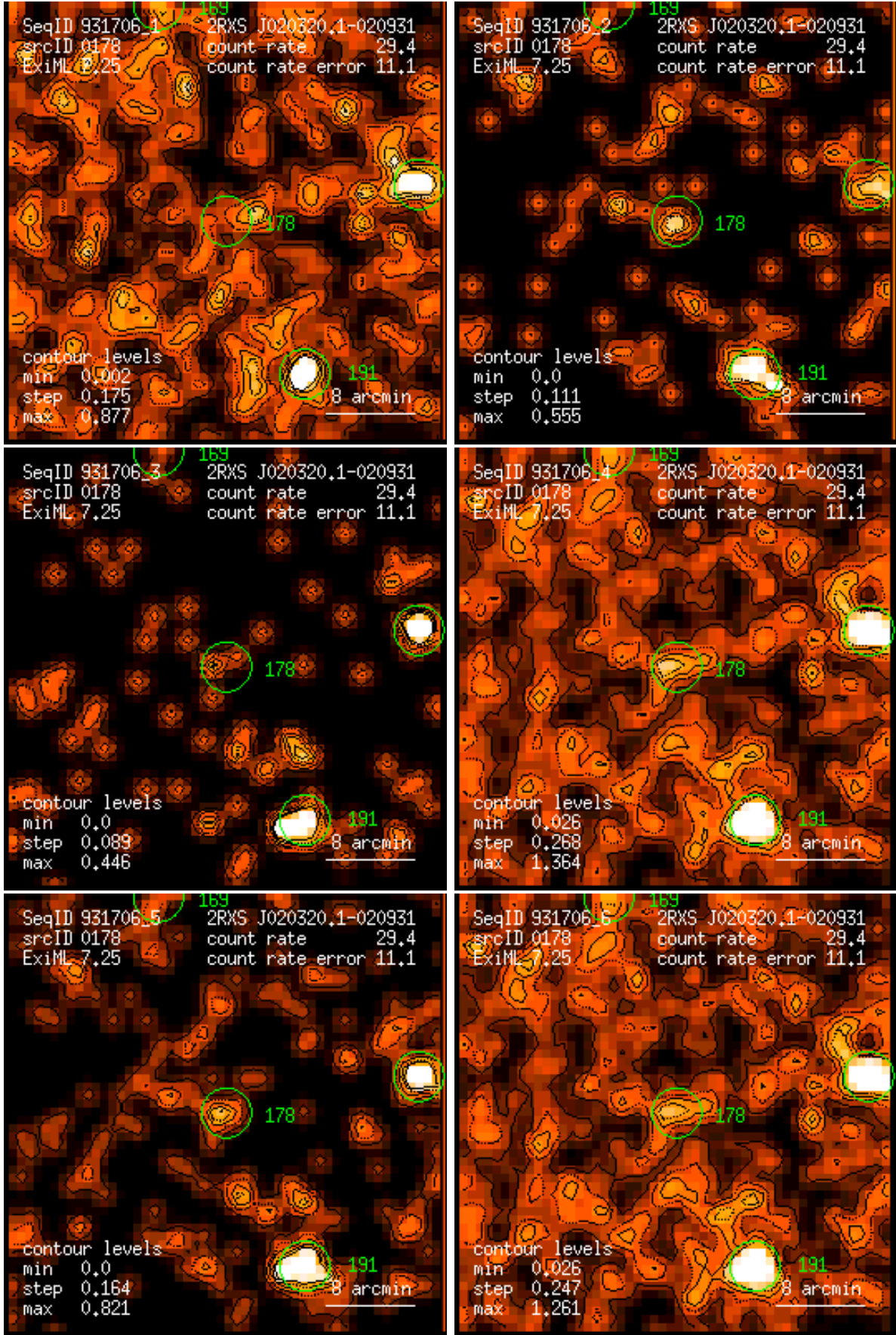
Figure 178: RASS 931706: detection 0178: band rate images, Gaussian filter: (1) PSPC channels 11 – 41, (2) 52 – 90, (3) 91 – 201, (4) 11 – 235, (5) 52 – 201, (6) 11 – 201. Broad band rates in counts/ks. Band rate contour levels in counts/ks/arcmin 2 .
