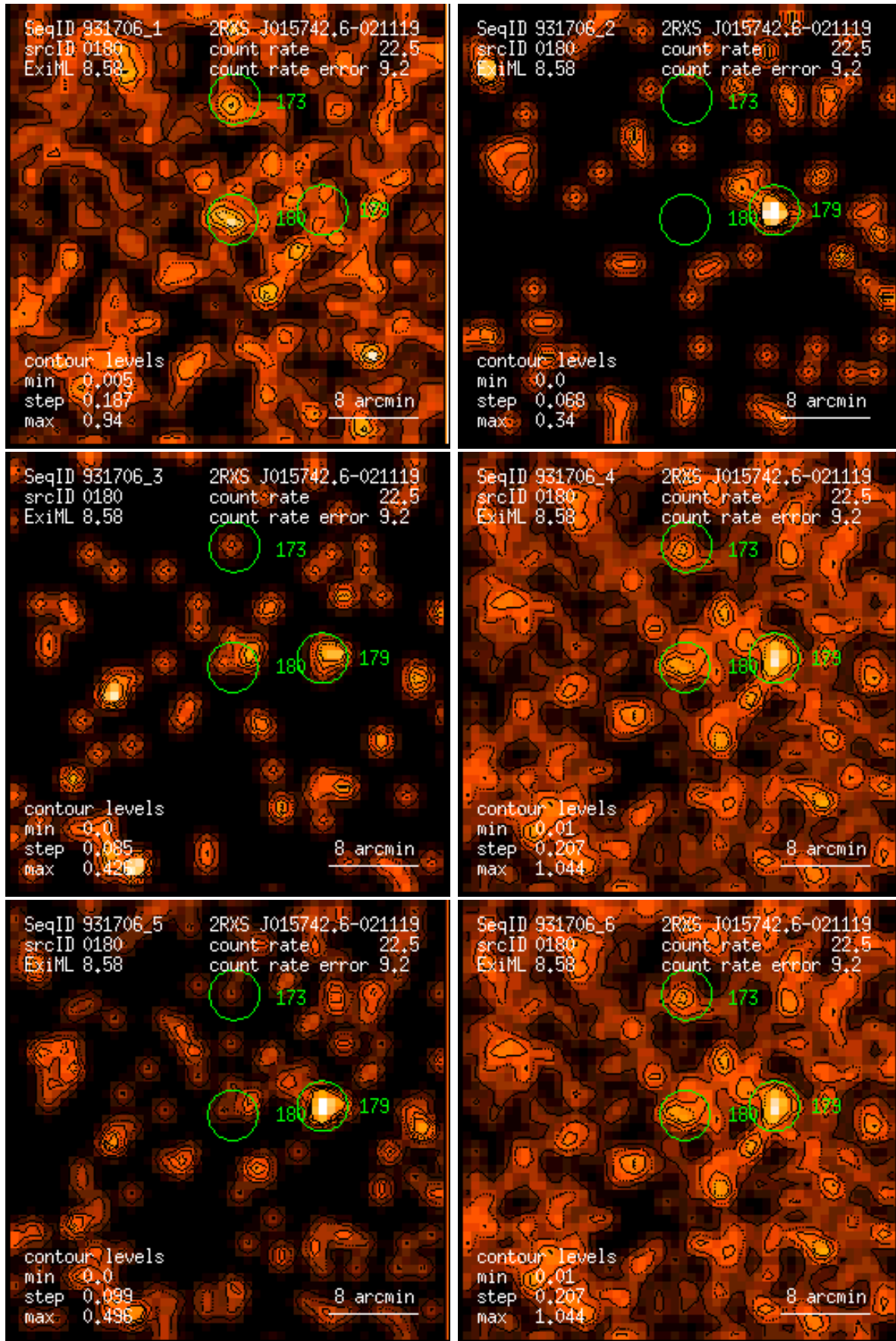
Figure 180: RASS 931706: detection 0180: band rate images, Gaussian filter: (1) PSPC channels 11 – 41, (2) 52 – 90, (3) 91 – 201, (4) 11 – 235, (5) 52 – 201, (6) 11 – 201. Broad band rates in counts/ks. Band rate contour levels in counts/ks/arcmin 2 .
