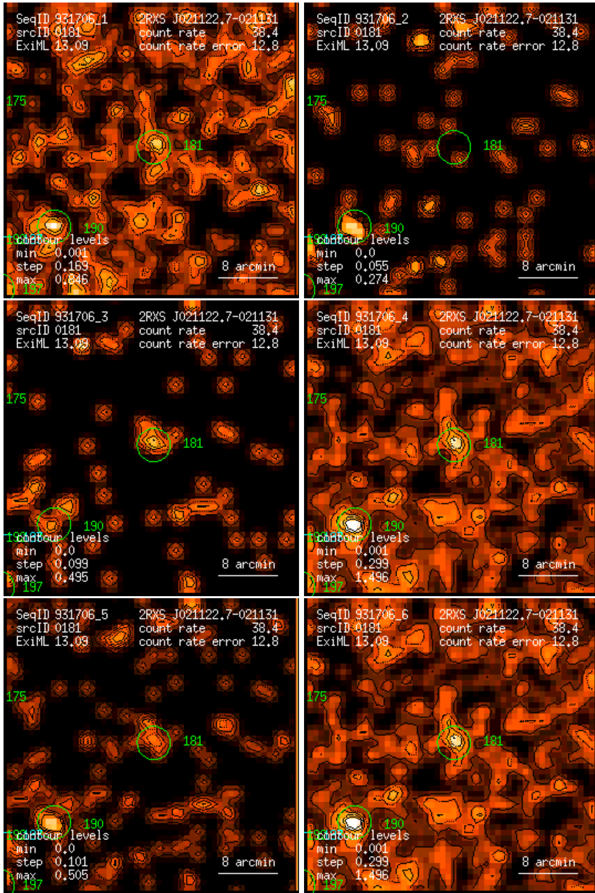
Figure 181: RASS 931706: detection 0181: band rate images, Gaussian filter: (1) PSPC channels 11 – 41, (2) 52 – 90, (3) 91 – 201, (4) 11 – 235, (5) 52 – 201, (6) 11 – 201. Broad band rates in counts/ks. Band rate contour levels in counts/ks/arcmin 2 .
