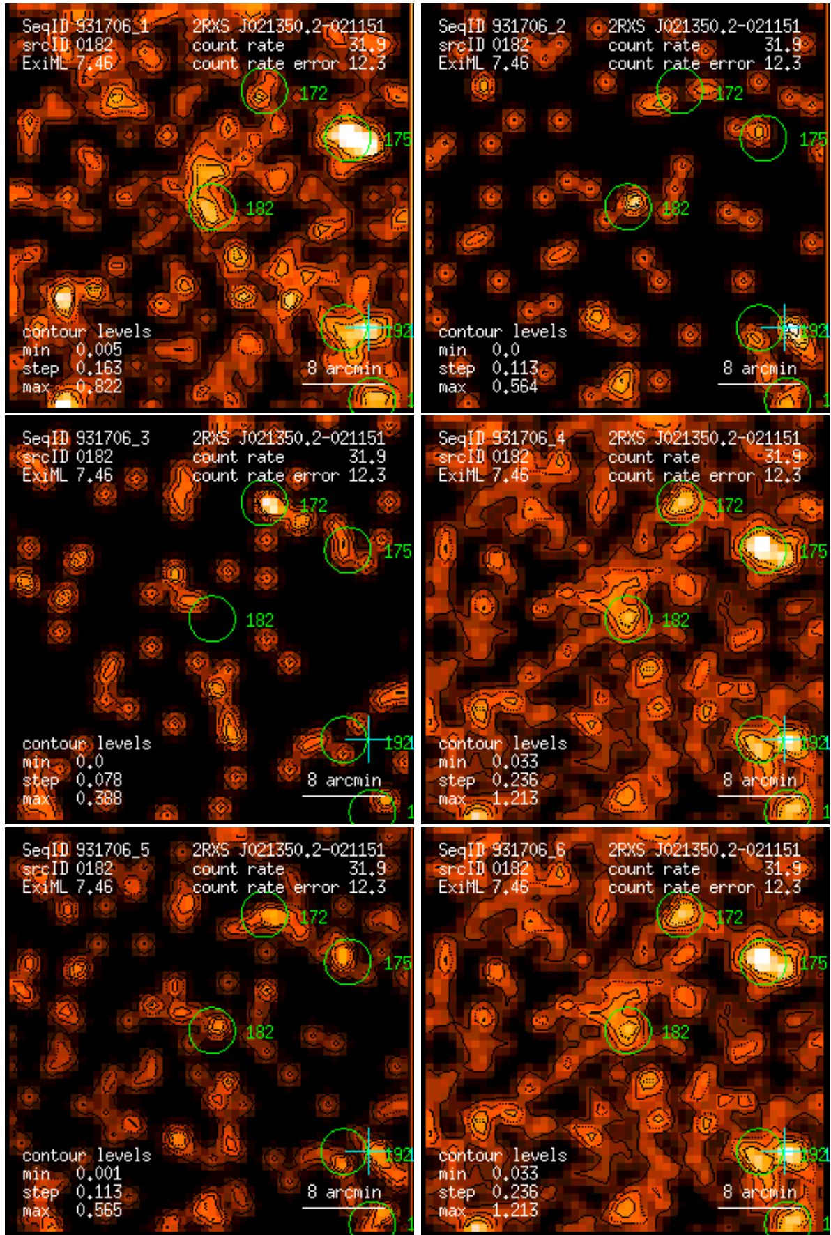
Figure 182: RASS 931706: detection 0182: band rate images, Gaussian filter: (1) PSPC channels 11 – 41, (2) 52 – 90, (3) 91 – 201, (4) 11 – 235, (5) 52 – 201, (6) 11 – 201. Broad band rates in counts/ks. Band rate contour levels in counts/ks/arcmin 2 .
