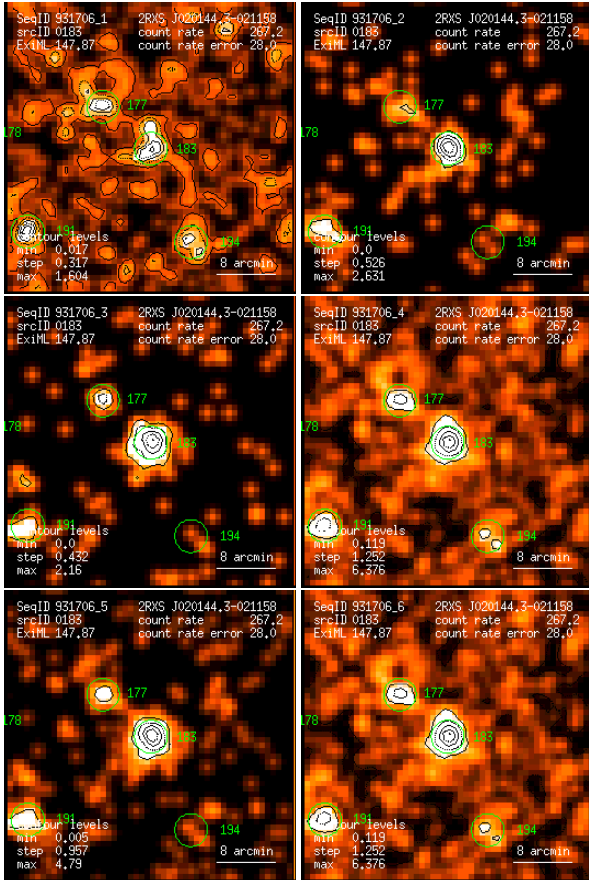
Figure 183: RASS 931706: detection 0183: band rate images, Gaussian filter: (1) PSPC channels 11 – 41, (2) 52 – 90, (3) 91 – 201, (4) 11 – 235, (5) 52 – 201, (6) 11 – 201. Broad band rates in counts/ks. Band rate contour levels in counts/ks/arcmin 2 .
