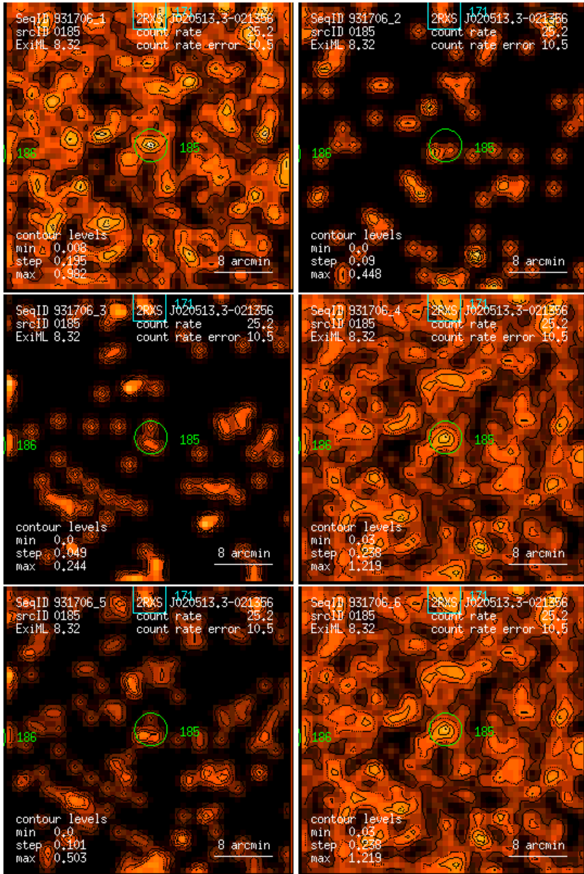
Figure 185: RASS 931706: detection 0185: band rate images, Gaussian filter: (1) PSPC channels 11 – 41, (2) 52 – 90, (3) 91 – 201, (4) 11 – 235, (5) 52 – 201, (6) 11 – 201. Broad band rates in counts/ks. Band rate contour levels in counts/ks/arcmin 2 .
