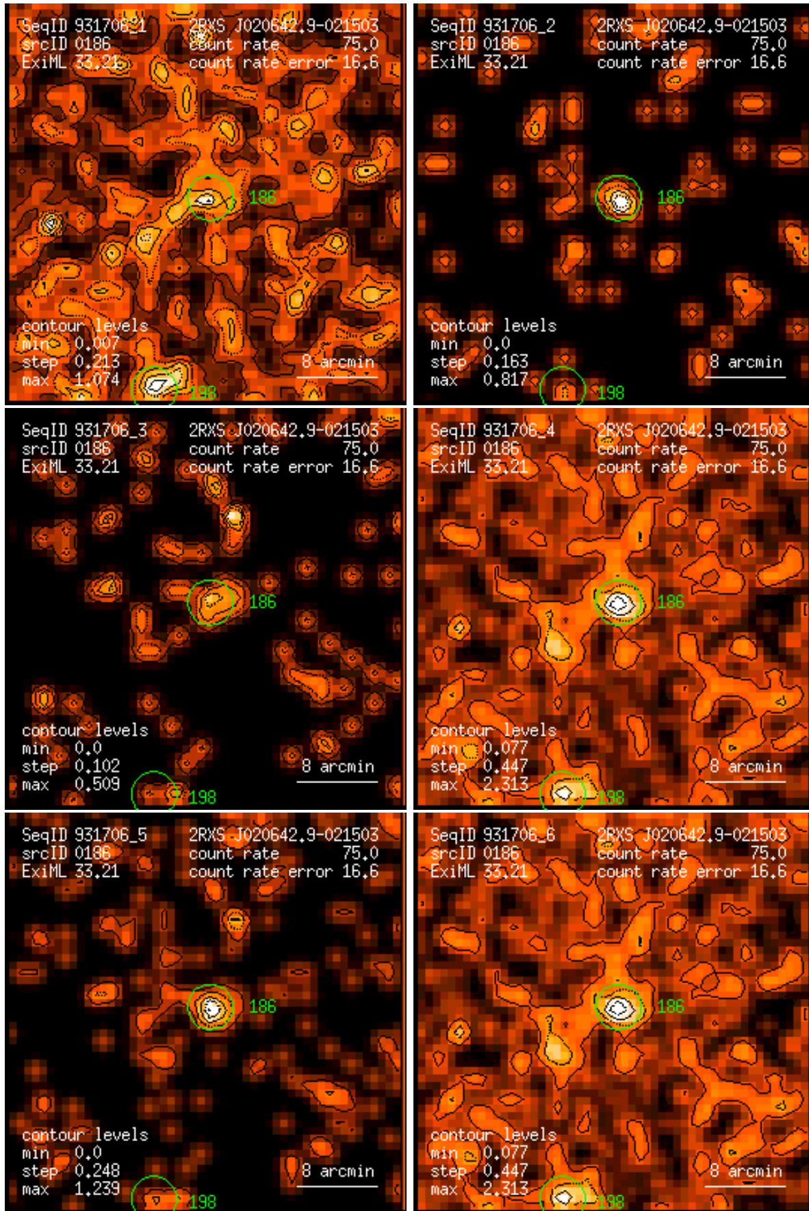
Figure 186: RASS 931706: detection 0186: band rate images, Gaussian filter: (1) PSPC channels 11 – 41, (2) 52 – 90, (3) 91 – 201, (4) 11 – 235, (5) 52 – 201, (6) 11 – 201. Broad band rates in counts/ks. Band rate contour levels in counts/ks/arcmin 2 .
