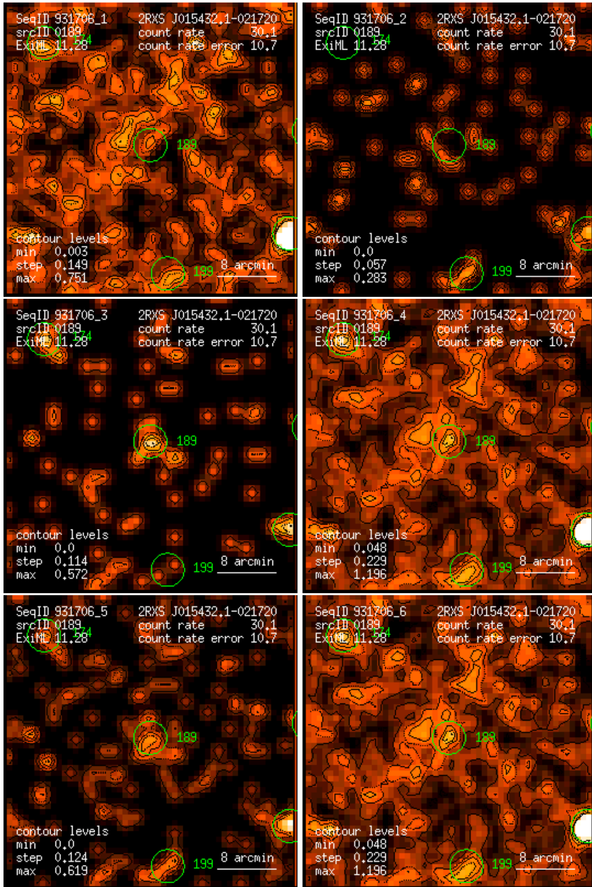
Figure 189: RASS 931706: detection 0189: band rate images, Gaussian filter: (1) PSPC channels 11 – 41, (2) 52 – 90, (3) 91 – 201, (4) 11 – 235, (5) 52 – 201, (6) 11 – 201. Broad band rates in counts/ks. Band rate contour levels in counts/ks/arcmin 2 .
