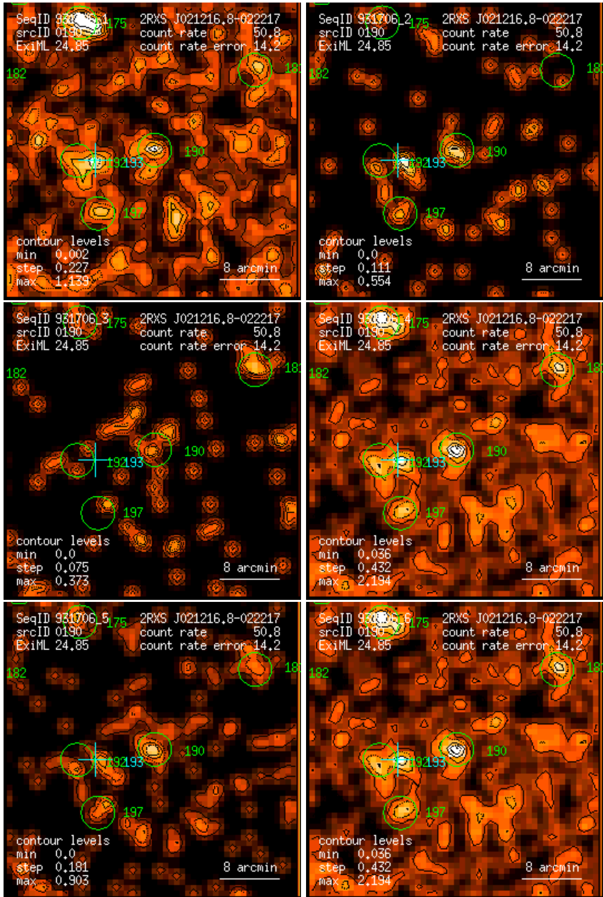
Figure 190: RASS 931706: detection 0190: band rate images, Gaussian filter: (1) PSPC channels 11 – 41, (2) 52 – 90, (3) 91 – 201, (4) 11 – 235, (5) 52 – 201, (6) 11 – 201. Broad band rates in counts/ks. Band rate contour levels in counts/ks/arcmin 2 .
