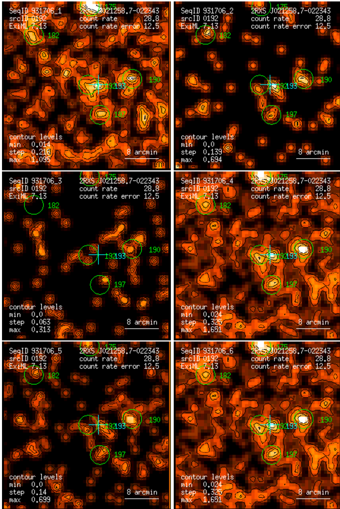
Figure 192: RASS 931706: detection 0192: band rate images, Gaussian filter: (1) PSPC channels 11 – 41, (2) 52 – 90, (3) 91 – 201, (4) 11 – 235, (5) 52 – 201, (6) 11 – 201. Broad band rates in counts/ks. Band rate contour levels in counts/ks/arcmin 2 .
