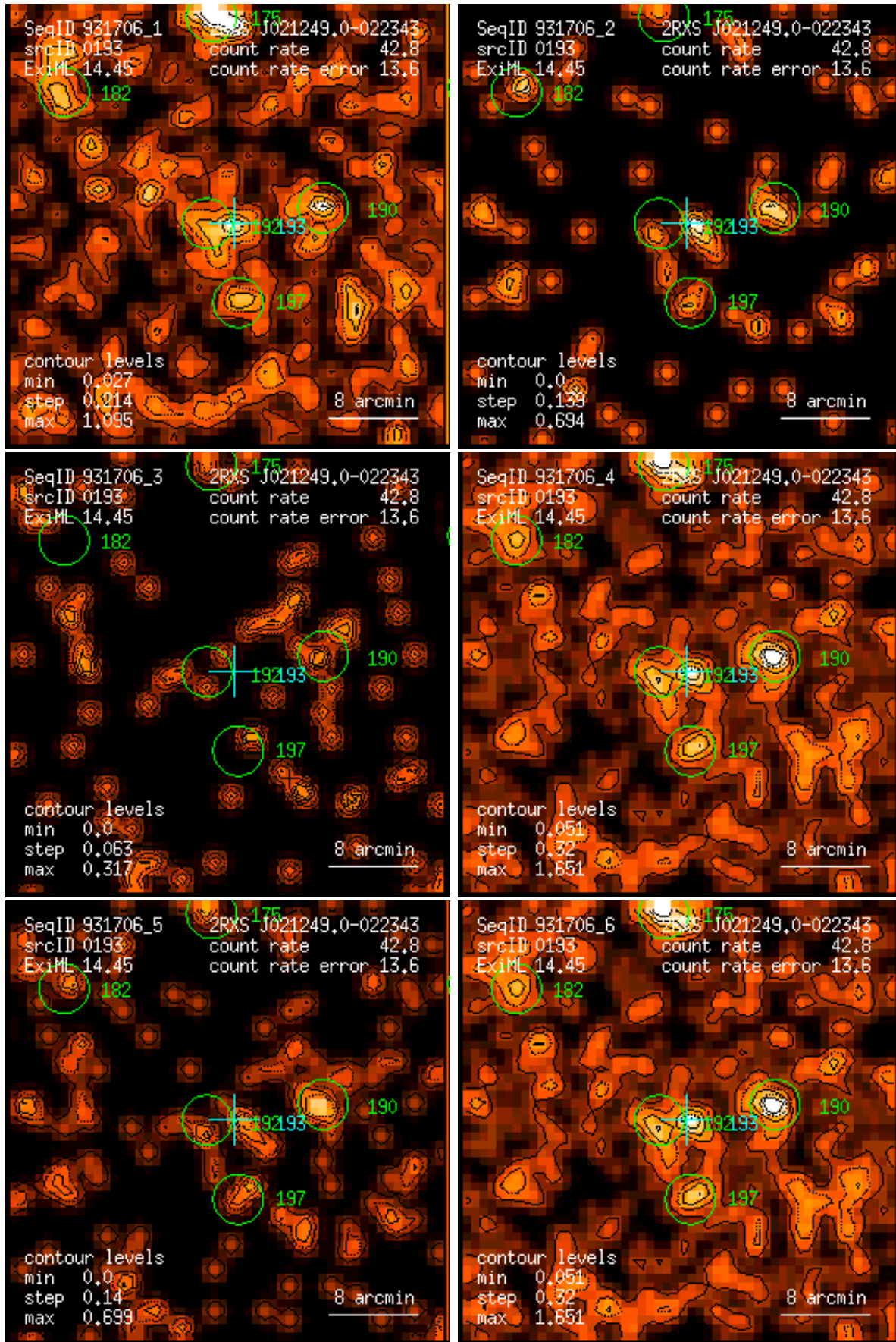
Figure 193: RASS 931706: detection 0193: band rate images, Gaussian filter: (1) PSPC channels 11 – 41, (2) 52 – 90, (3) 91 – 201, (4) 11 – 235, (5) 52 – 201, (6) 11 – 201. Broad band rates in counts/ks. Band rate contour levels in counts/ks/arcmin 2 .
