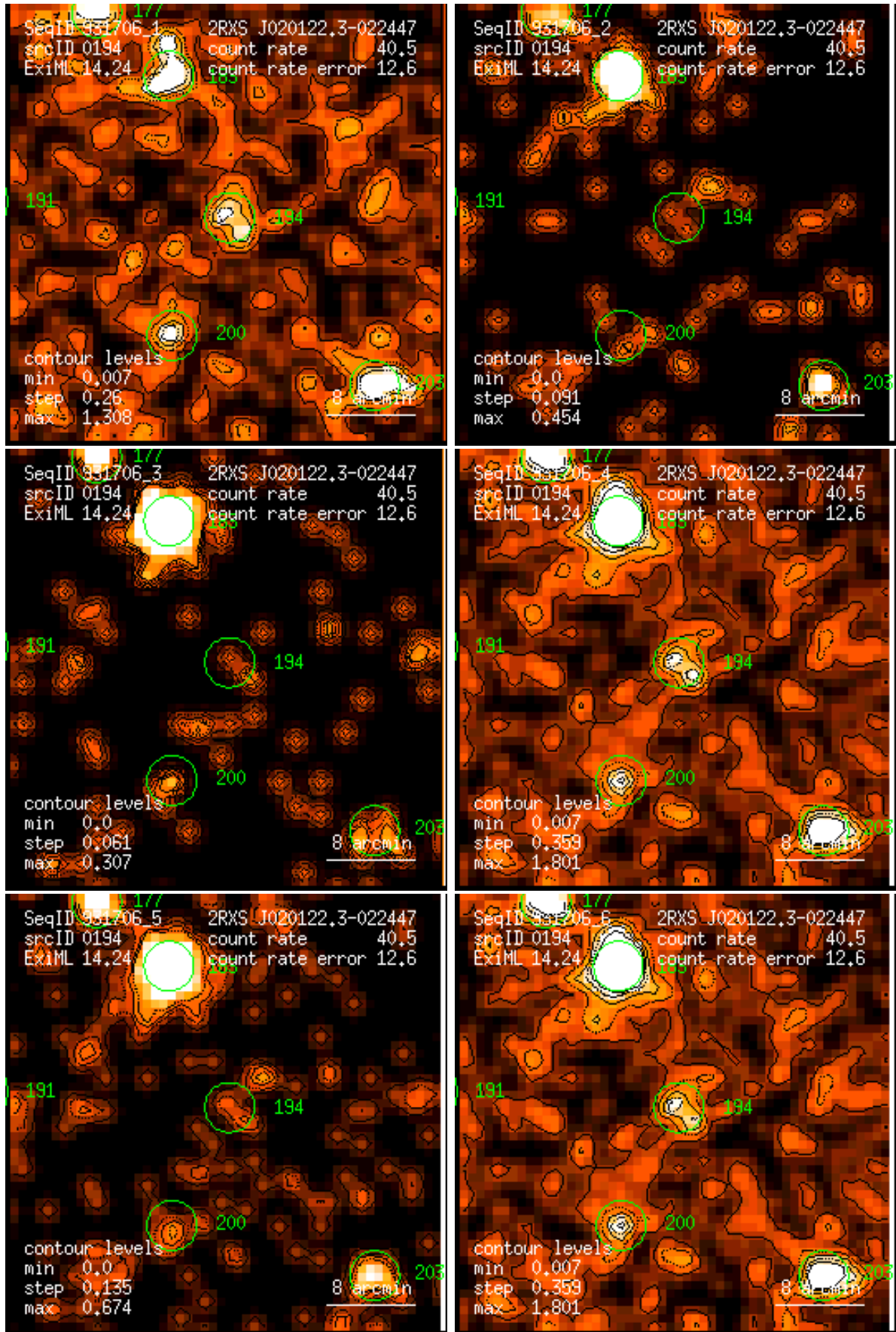
Figure 194: RASS 931706: detection 0194: band rate images, Gaussian filter: (1) PSPC channels 11 – 41, (2) 52 – 90, (3) 91 – 201, (4) 11 – 235, (5) 52 – 201, (6) 11 – 201. Broad band rates in counts/ks. Band rate contour levels in counts/ks/arcmin 2 .
