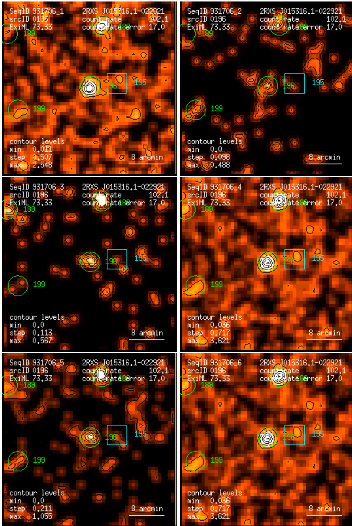
Figure 196: RASS 931706: detection 0196: band rate images, Gaussian filter: (1) PSPC channels 11 – 41, (2) 52 – 90, (3) 91 – 201, (4) 11 – 235, (5) 52 – 201, (6) 11 – 201. Broad band rates in counts/ks. Band rate contour levels in counts/ks/arcmin 2 .
