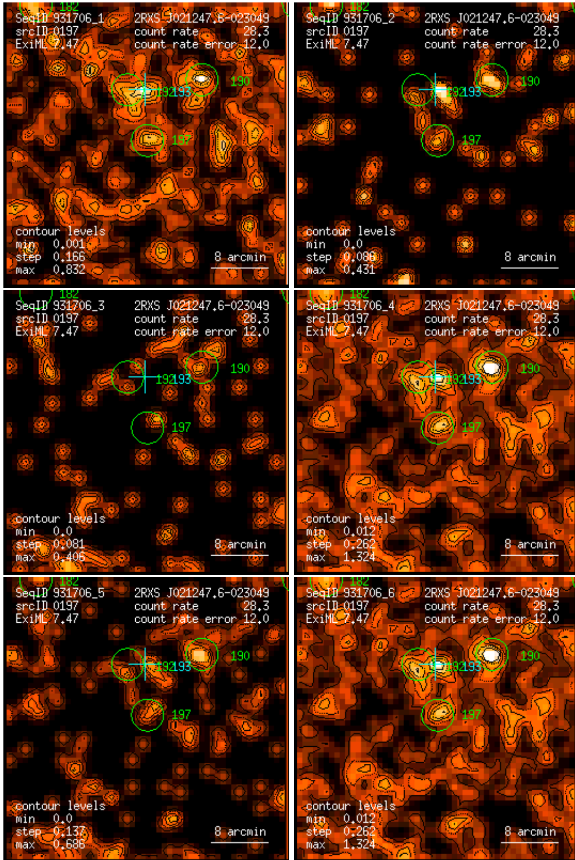
Figure 197: RASS 931706: detection 0197: band rate images, Gaussian filter: (1) PSPC channels 11 – 41, (2) 52 – 90, (3) 91 – 201, (4) 11 – 235, (5) 52 – 201, (6) 11 – 201. Broad band rates in counts/ks. Band rate contour levels in counts/ks/arcmin 2 .
