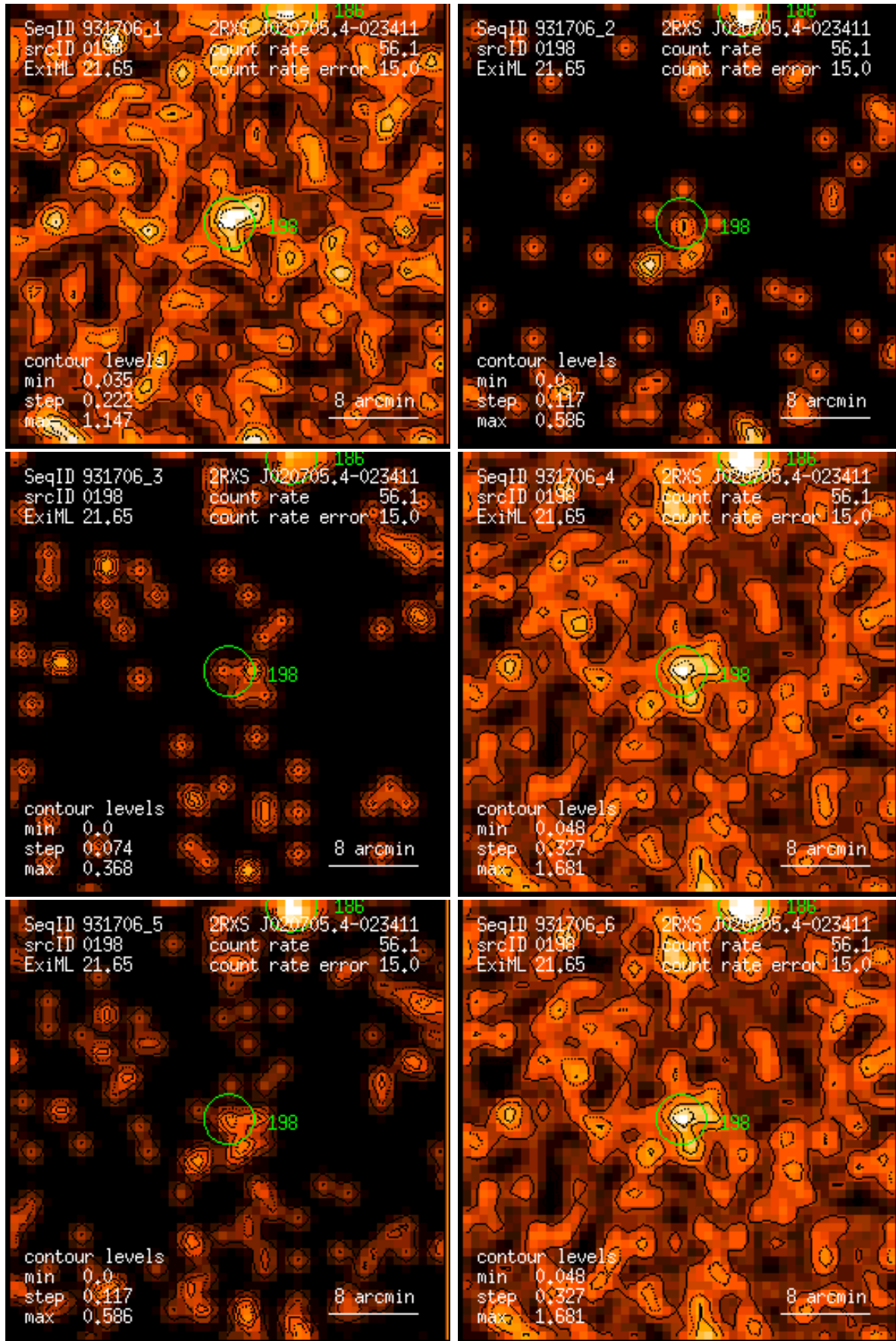
Figure 198: RASS 931706: detection 0198: band rate images, Gaussian filter: (1) PSPC channels 11 – 41, (2) 52 – 90, (3) 91 – 201, (4) 11 – 235, (5) 52 – 201, (6) 11 – 201. Broad band rates in counts/ks. Band rate contour levels in counts/ks/arcmin 2 .
