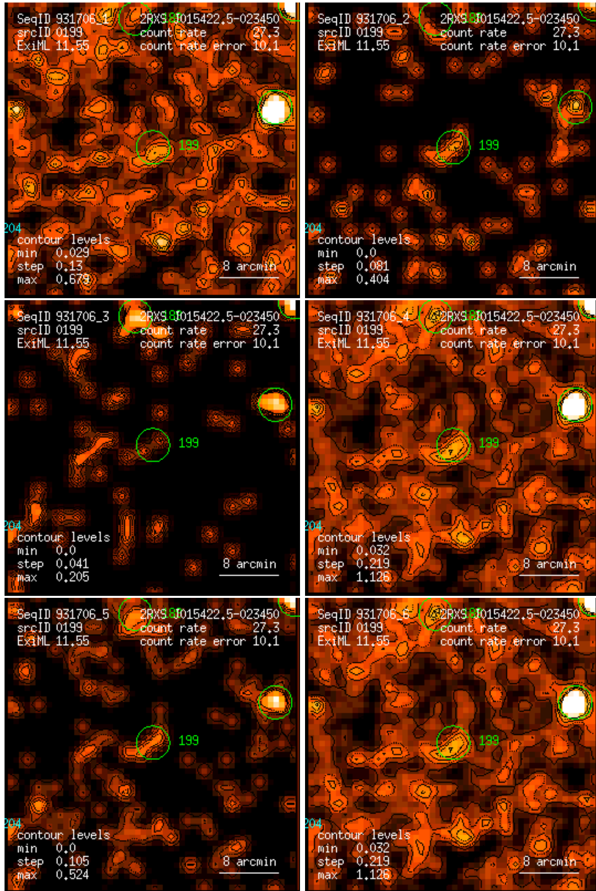
Figure 199: RASS 931706: detection 0199: band rate images, Gaussian filter: (1) PSPC channels 11 – 41, (2) 52 – 90, (3) 91 – 201, (4) 11 – 235, (5) 52 – 201, (6) 11 – 201. Broad band rates in counts/ks. Band rate contour levels in counts/ks/arcmin 2 .
