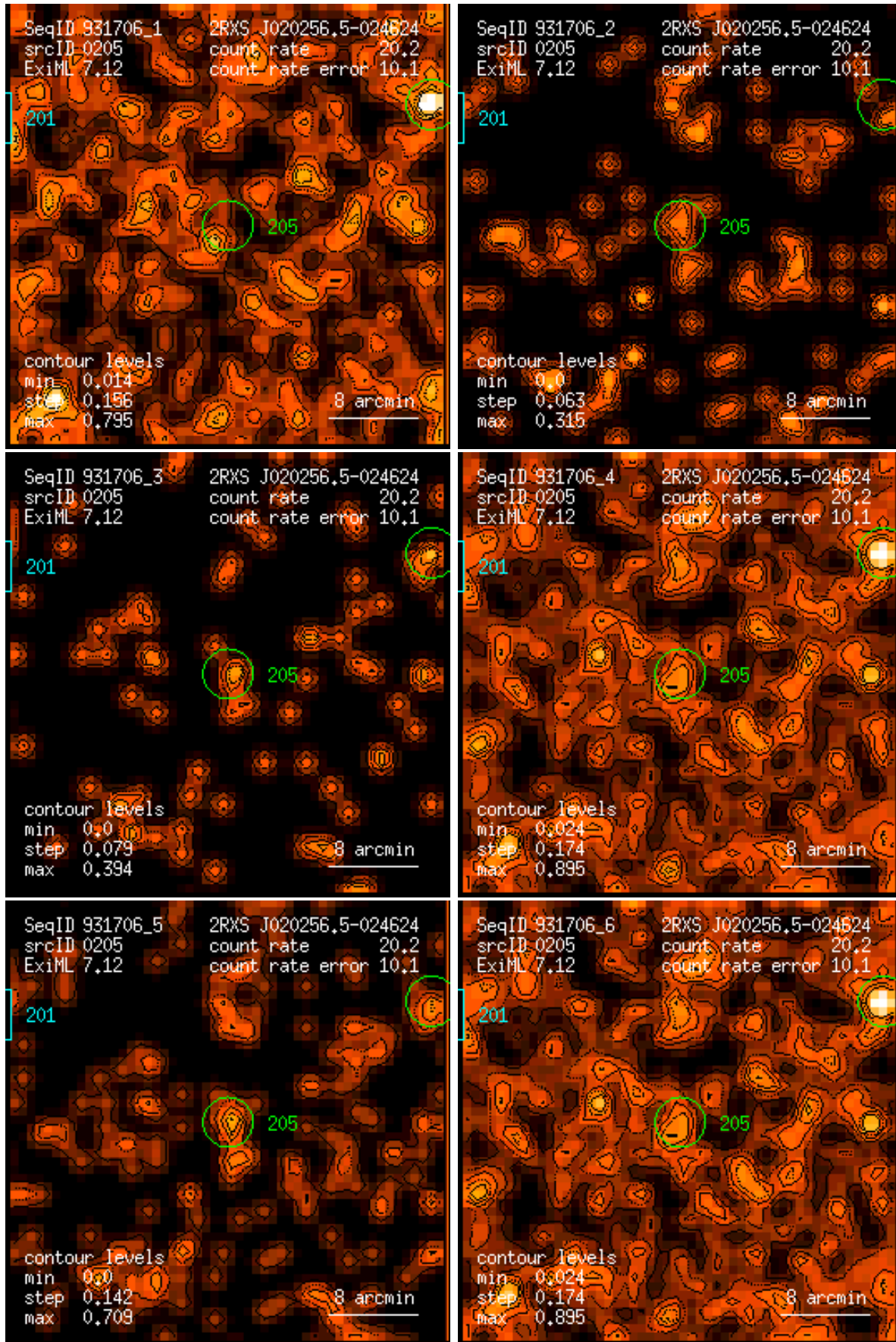
Figure 205: RASS 931706: detection 0205: band rate images, Gaussian filter: (1) PSPC channels 11 – 41, (2) 52 – 90, (3) 91 – 201, (4) 11 – 235, (5) 52 – 201, (6) 11 – 201. Broad band rates in counts/ks. Band rate contour levels in counts/ks/arcmin 2 .
