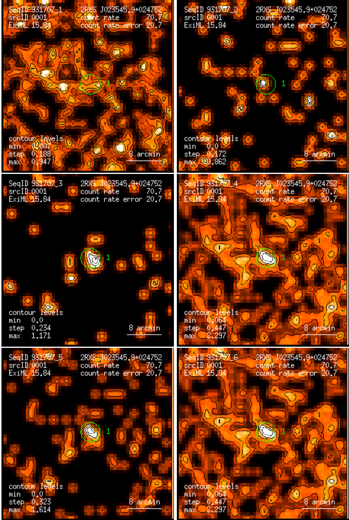
Figure 1: RASS 931707: detection 0001: band rate images, Gaussian filter: (1) PSPC channels 11 – 41, (2) 52 – 90, (3) 91 – 201, (4) 11 – 235, (5) 52 – 201, (6) 11 – 201. Broad band rates in counts/ks. Band rate contour levels in counts/ks/arcmin 2 .
