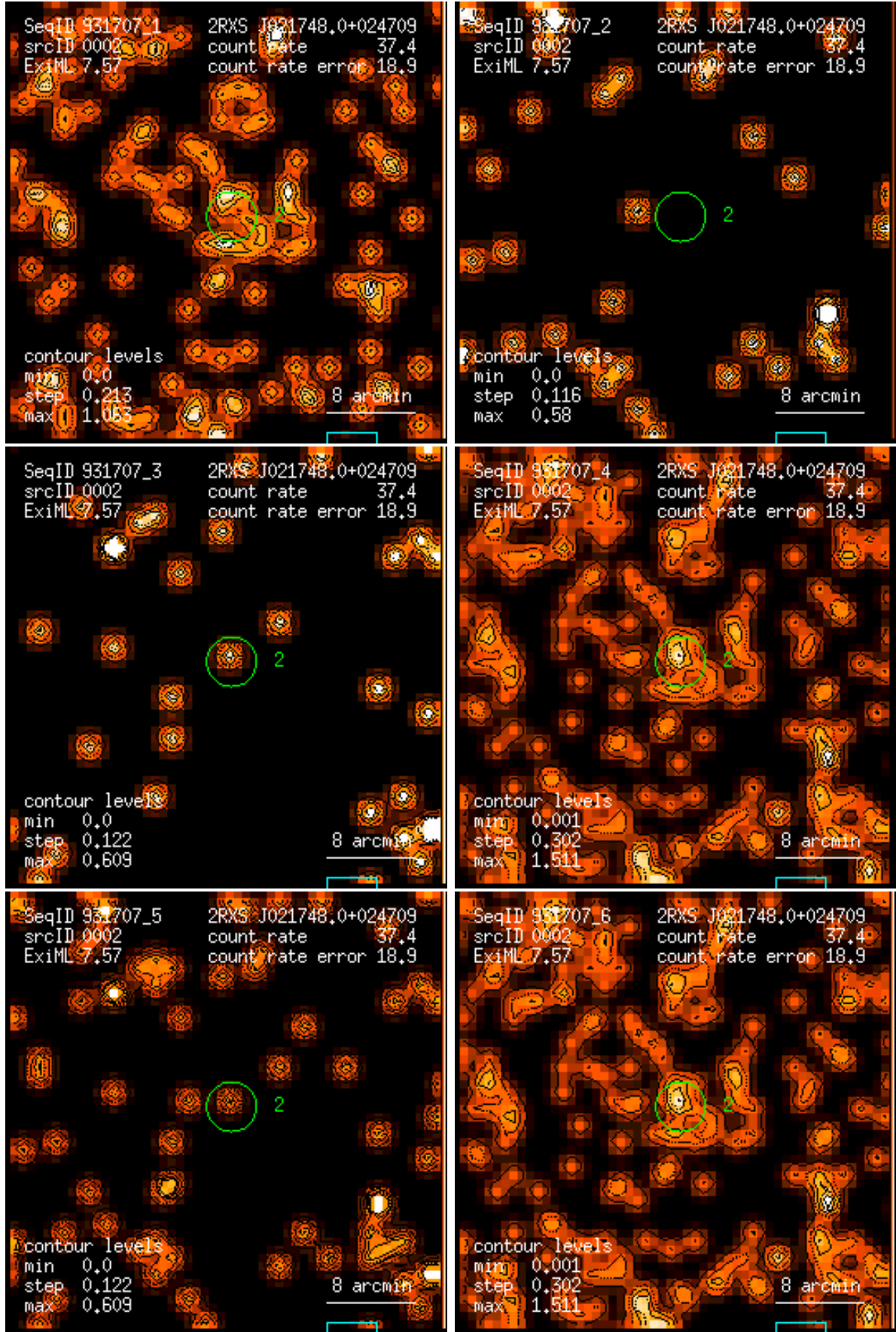
Figure 2: RASS 931707: detection 0002: band rate images, Gaussian filter: (1) PSPC channels 11 – 41, (2) 52 – 90, (3) 91 – 201, (4) 11 – 235, (5) 52 – 201, (6) 11 – 201. Broad band rates in counts/ks. Band rate contour levels in counts/ks/arcmin 2 .
